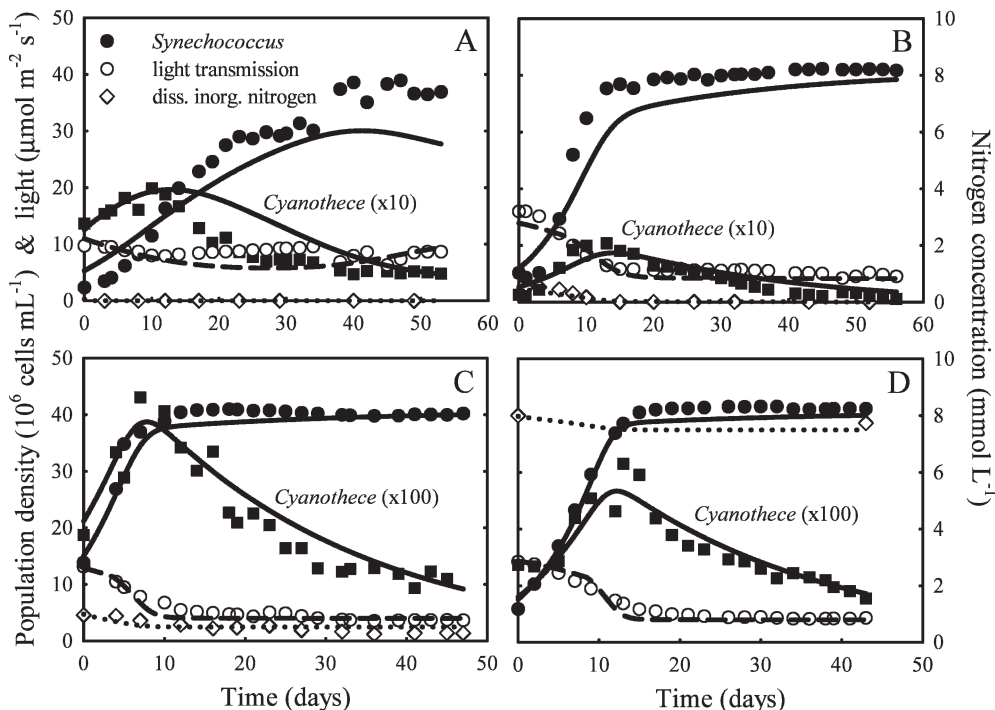
Fig. 7. Competition experiments between the picocyanobacterium Synechococcus and the nitrogen-fixing cyanobacterium Cyanothece at low light ( I_m = 20 \mu mol m^{-2} s^{-1} ). (A) Synechococcus (closed circles) and Cyanothece (squares) coexist at low nitrate input ( R_m = 0.1 mmol L^{-1} ). (B–D) Synechococcus (closed circles) displaces Cyanothece (squares) at (B) low-intermediate nitrate input ( R_m = 0.5 mmol L^{-1} ), (C) intermediate nitrate input ( R_m = 1 mmol L^{-1} ), and (D) high nitrate input ( R_m = 8 mmol L^{-1} ). Open circles indicate the light intensity I_{out} transmitted through the cultures, and diamonds indicate the concentration of dissolved inorganic nitrogen (the sum of nitrate, nitrite, and ammonium). Lines represent model predictions of population density (solid lines), transmitted light (dashed lines), and dissolved inorganic nitrogen (dotted lines). System parameters and initial conditions are given in Table 1, and parameter values of Synechococcus and Cyanothece are given in Table 3. Note that the population density of Cyanothece is magnified by a factor 10 in (A) and (B), and by a factor 100 in (C) and (D).
