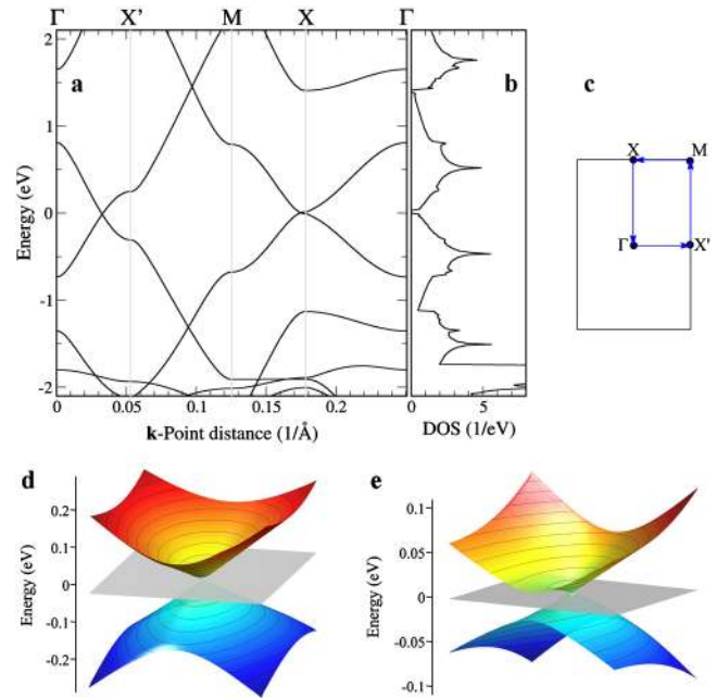
FIG. 4 (color online). Electronic structure of 6,6,12-graphyne. (a) Band structure. The two different Dirac points are labeled by I and II. (b) DOS. (c) First Brillouin zone with letters designating special points and with the lines along which the band structure is displayed. (d) Dirac cone I. (e) Dirac cone II. Gray planes in panels (d) and (e) indicate the Fermi level.
