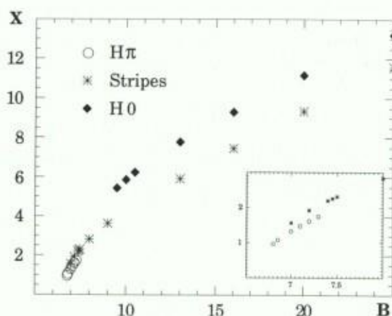
Fig. 2. Bifurcation diagram compiled from the numerical simulations using set I of parameters. [X_{\max} - X_0] is drawn as a function of the bifurcation parameter B . The inset zooms in the region near B_c .
