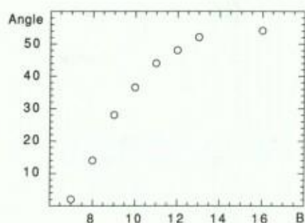
Fig. 4. Bifurcation diagram representing the size of the knee angle of the zig-zig stripes as a function of B for set 1 of parameters.
