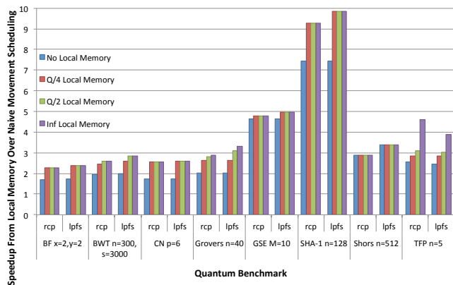
Figure 8: Speedups due to the addition of local memory to operating regions, computed over a sequential, naive movement model. Results are shown for a Multi-SIMD(4,∞) architecture.
