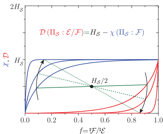
Figure 3 | Anti-symmetry of discord and the Holevo quantity for a pure \mathcal{SE} state and rank one POVM \Pi_S . This symmetry relates discord between \Pi_S and the remainder of the environment \mathcal{E}/\mathcal{F} and the Holevo quantity between \Pi_S and fragment \mathcal{F} . As the Holevo quantity increases – i.e., as the classical information transmitted by the environment increases – the discord on the opposite side of the axis decreases. Since the discord is monotonically increasing with f , this means that the quantum information about S is pushed into correlations with the global environment as redundant (classical) information is increased. Thus, a state which has redundant information will have quantum information encoded in the environment, implying that Quantum Darwinism is in action.
