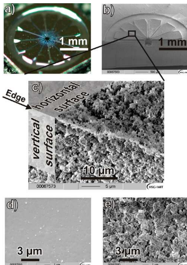
Figure 1. (a) Star-shaped structure fabricated in silicon. (b) The cut chip of PTFE/PDMS composite. (c) SEM picture of an edge showing horizontal and vertical surface. (d) Untreated surface of sample with 15 wt % PTFE particles. (e) Plasma-treated surface of sample with 15 wt % PTFE particles.
