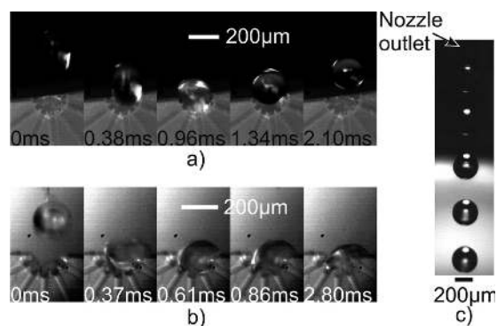
Figure 3. (a) Water droplet dispensed onto the cut structure of the completely superhydrophobic PDMS/PTFE chip, viewed from direction A (refer to Figure 2f). (b) Water droplet dispensed onto an identical structure in an intrinsic PDMS chip. (c) Application of the completely superhydrophobic nozzle for continuous dispensing of water drops.
