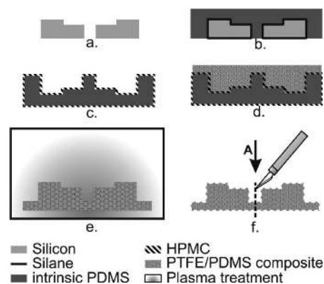
Figure 2. Fabrication steps of a completely superhydrophobic PDMS chip.
