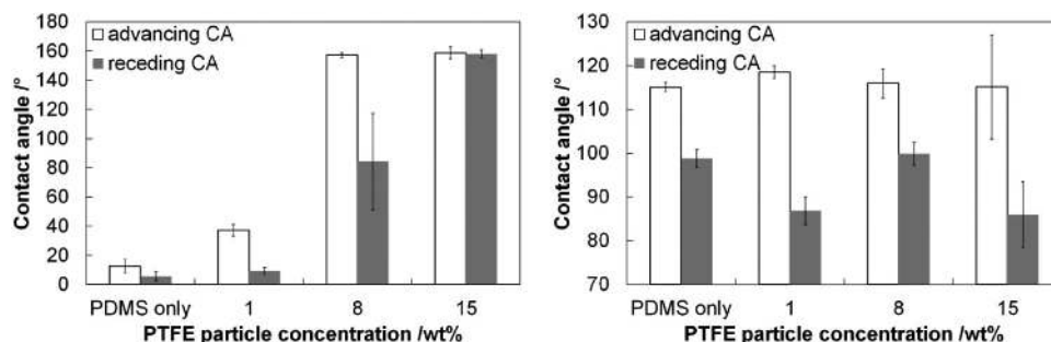
Figure 4. Contact angle measurements on the plasma-modified samples (left) and untreated samples (right).
