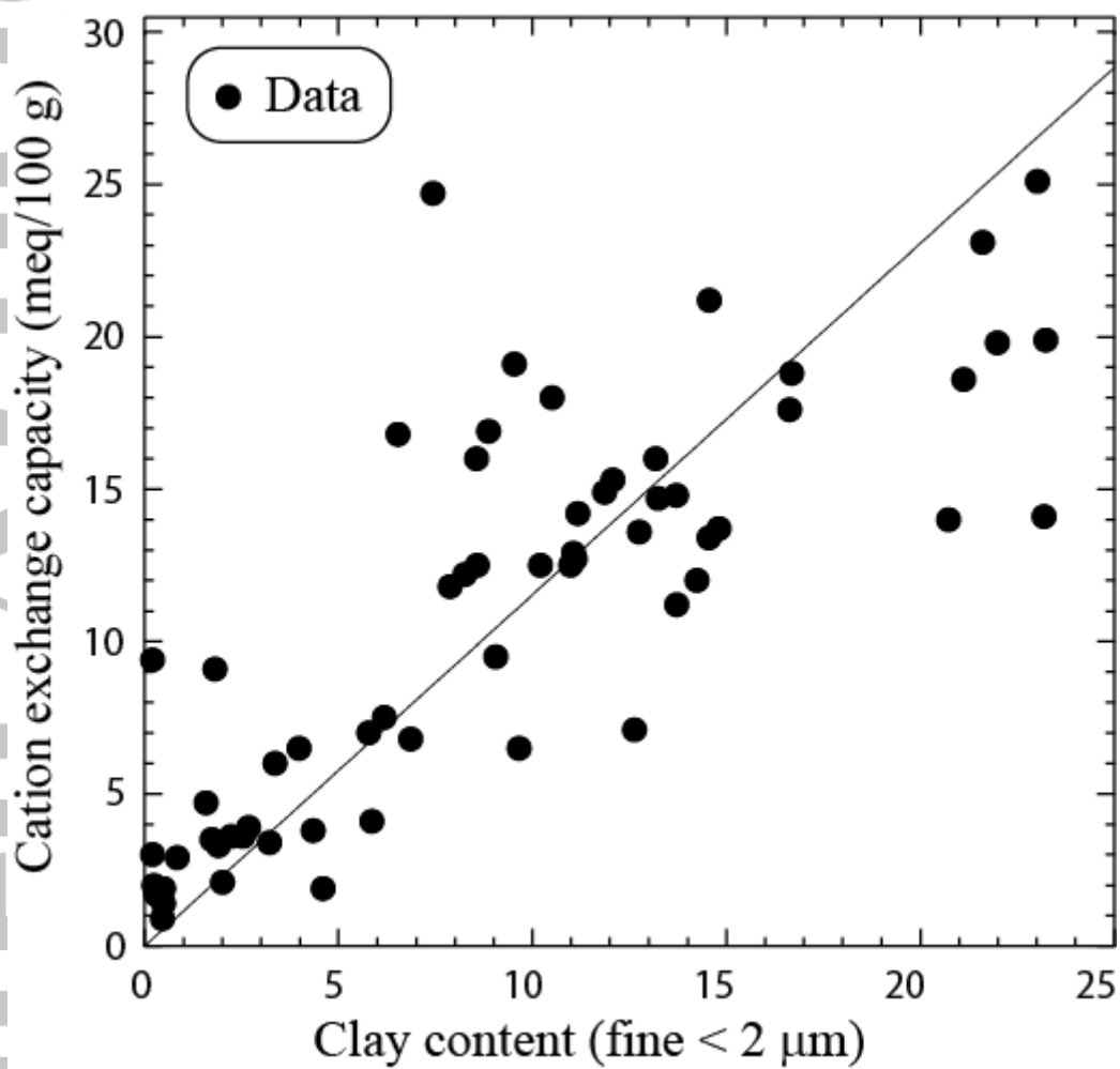
Figure 9. Relationship between the cation exchange capacity (CEC) and the clay content taken as the weight fraction of fine particles smaller than 2 μm. The data are scattered because of the effect of humus and variations between the core sample in the clay mineralogy.
