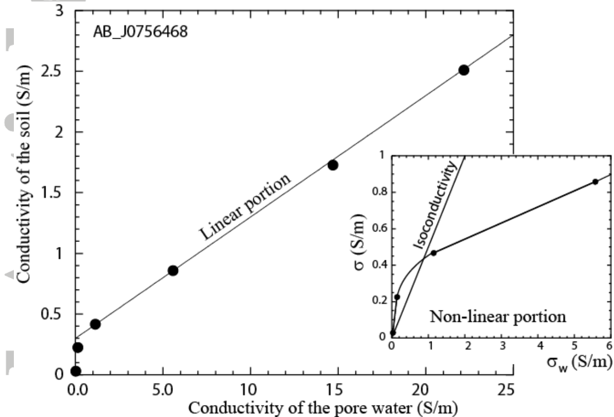
Figure 10. Conductivity versus pore water conductivity showing the linear (obeying to equation 5) and non-linear portions of the conductivity plot. The non-linear portion at low salinities is due to a change in the tortuosity of the conduction paths. The quantities \sigma and \sigma_w define the conductivity of the soil and the conductivity of the pore water.
