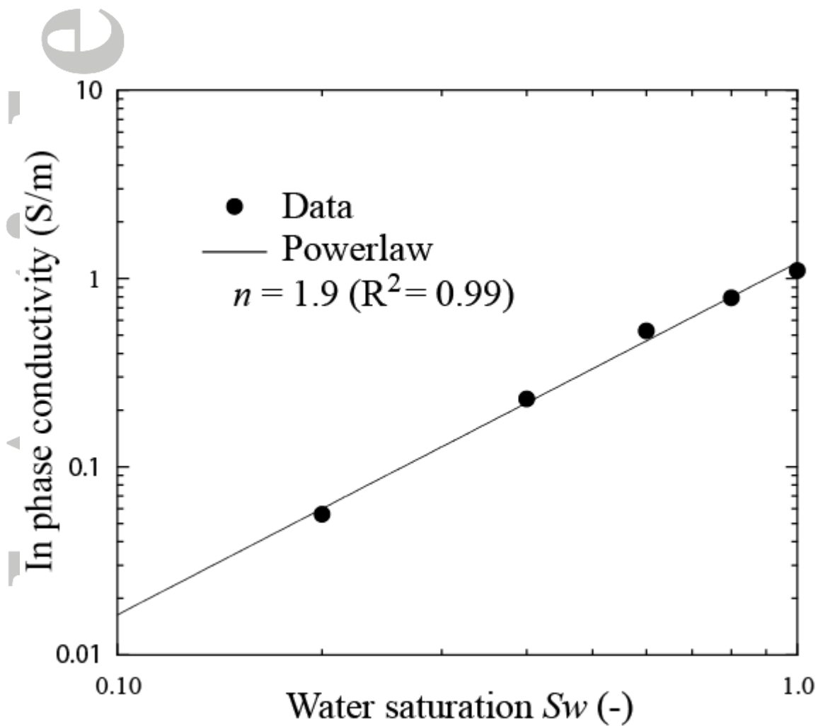
Figure 24. Saturation dependence of the in phase conductivity (1 Hertz)) at high salinity (NaCl solution at 5 \text{ S m}^{-1} , sample BB, fine sand). The dependence is used to determine the second Archie's exponent n .
