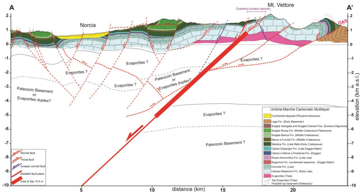
Figure 9: Geological cross-section A-A', orthogonal to the modelled N155° fault (from 1:10,000-scale cartography of Regione Umbria and Marche and Pierantoni et al., 2013) (trace in Fig. 1a). This section intersects the faults bounding the Norcia and Castelluccio basins and further to NE the OAS. The location and geometry of the modelled fault is reported along with its section of coseismic slip >0.5 m (thick red segment). In this interpretation, the shallow splays of the VBFS that ruptured at the surface during the October 30 th earthquake merge into the N155° fault between 1-2 km depth from the surface. The interpretation of the deeper setting is speculative.
