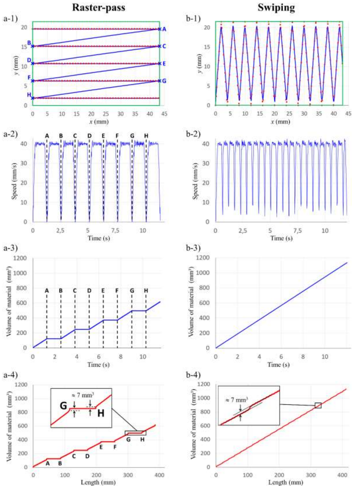
Fig. 6 Trajectory, speed and volume of materials for the raster-pass and swiping strategies, with a nominal speed of 40 mm/s
