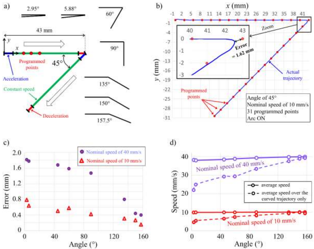
Fig. 4 Influence of the angle on a toolpath direction change: a) different angles considered and schematic representation for 45°, b) example of actual toolpath and definition of the error, c) error vs. angle for two nominal speeds of the robot, d) actual speeds achieved by the robot
