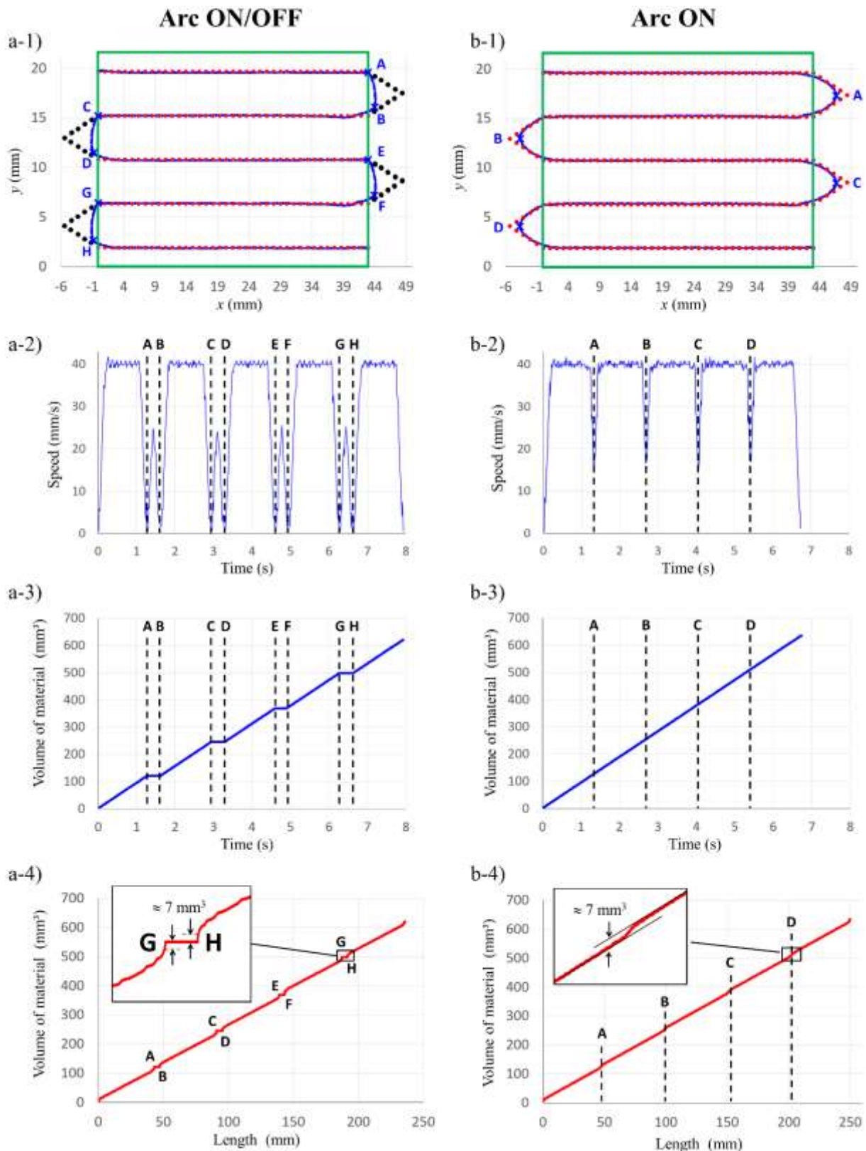
Fig. 7 Influence of the arc ON/OFF command on the trajectory for the 45° triangular and a nominal speed of 40 mm/s: a) with arc ON and OFF inside and outside the objective rectangle respectively, b) with arc ON activated over the whole toolpath
