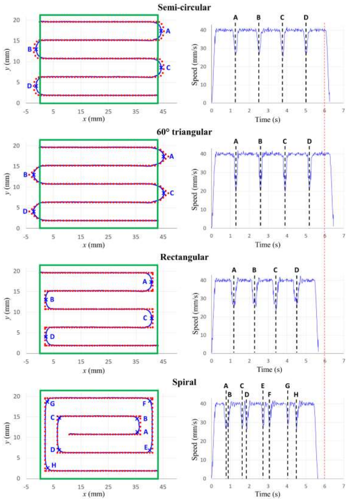
Fig. 5 Toolpath and speed for the semi-circular, rectangular and spiral strategies, as well as for one of the triangular strategies (namely 60°). The nominal speed was set to 40 mm/s and arc ON was activated over the whole of each trajectory
