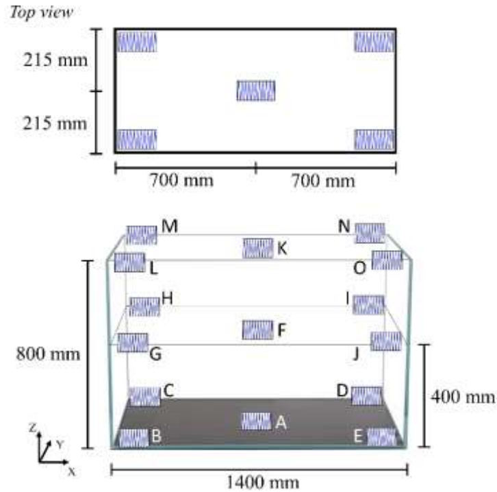
Fig. 8 Schematic view of the inert chamber with the locations of the different zones in which the same swiping depositions were performed
