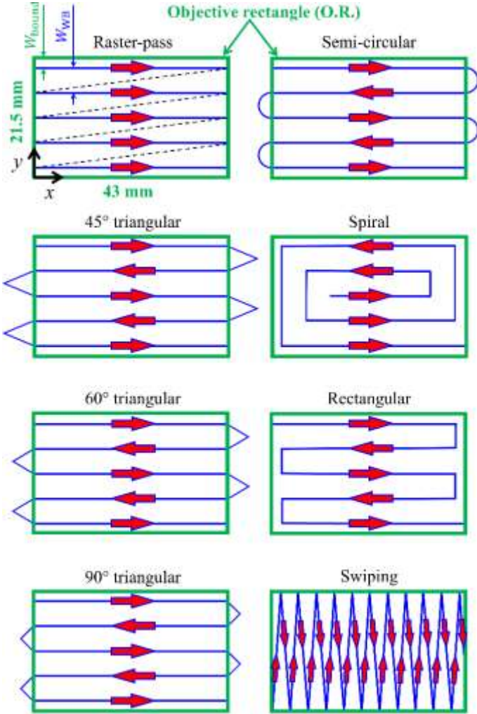
Fig. 2 Different strategies considered in the study
