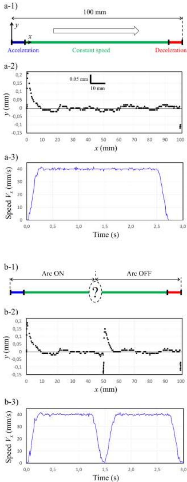
Fig. 3 Illustration of the influence of the arc ON/OFF command on the toolpath for a linear trajectory at a nominal speed of 40 mm/s: a) without changing the command, b) changing arc ON to arc OFF in the middle of the trajectory
