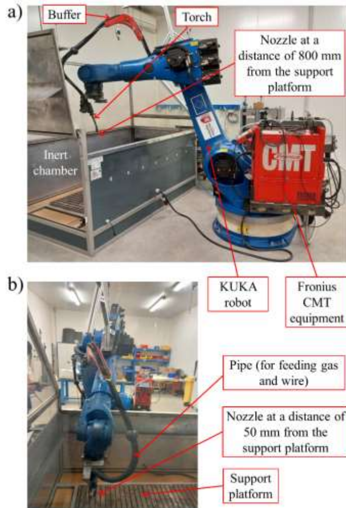
Fig. 1 Photos of the system. In the framework of this study, the nozzle movement was studied without activating the torch (trajectory definition only)
