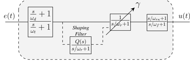
(b) Block diagram for approximating \left(\frac{s}{\omega_d} + 1\right) \left(\frac{s}{\omega_t} + 1\right)^{-\beta} . Approximation will be done in the range of [\omega_l, \omega_h] .
