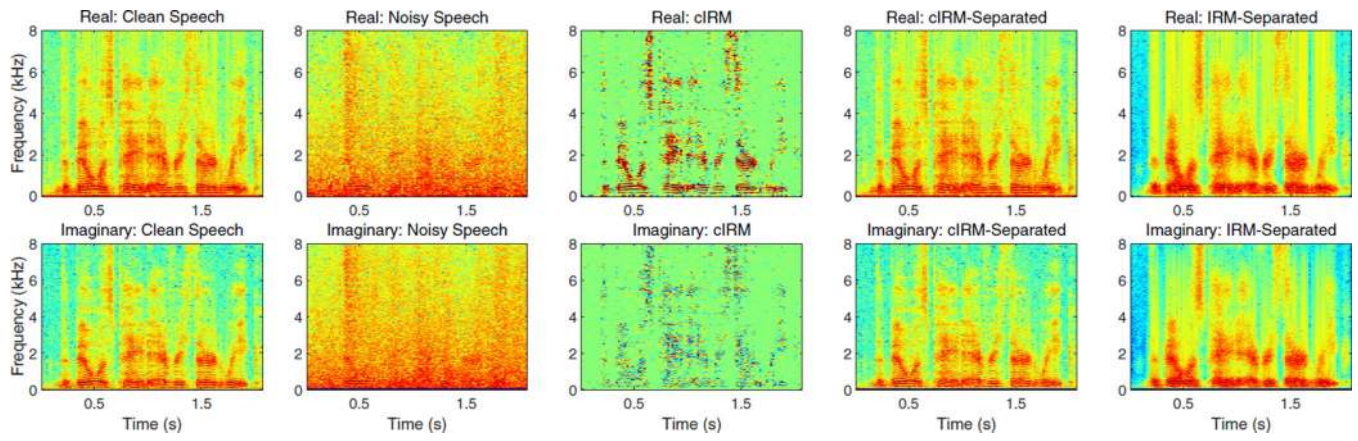
Fig. 2. (Color online) Spectrogram plots of the real (top) and imaginary (bottom) STFT components of clean speech, noisy speech, the complex ideal ratio mask, and speech separated with the complex ideal ratio mask and the ideal ratio mask.
