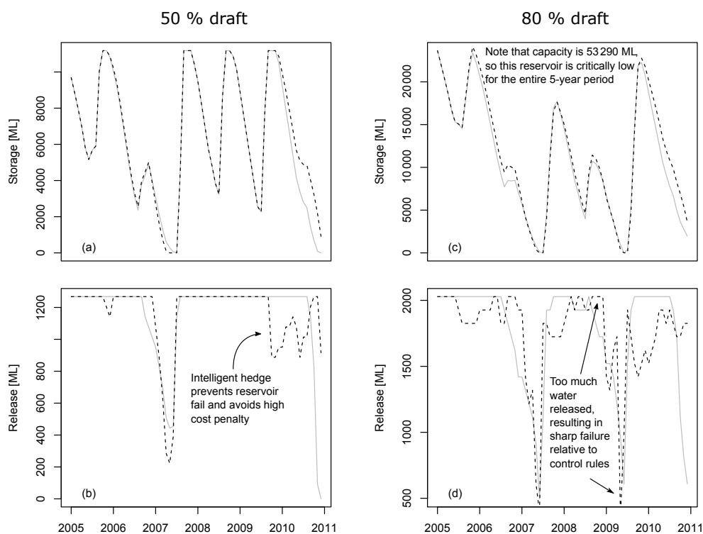
Figure 7. Storage and release time series for reservoirs in the Serpentine catchment with 50 % (a, b) and 80 % (c, d) draft ratios. The solid grey line gives operation under control rules whilst the dotted black line gives operation with the FoGSS forecast (median of ensemble).
