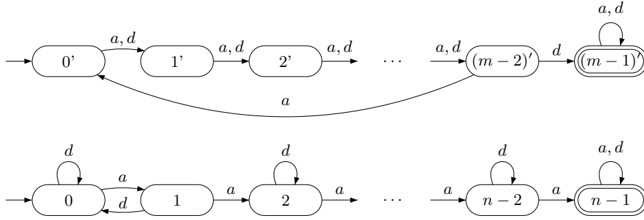
Figure 7: DFAs of L'_m(a, -, -, d) and L_n(-, -, d, a) for boolean operations.
