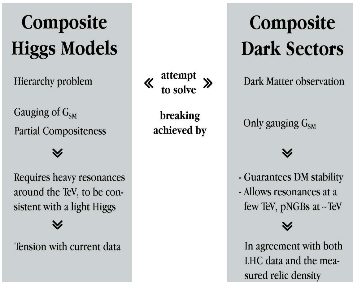
Figure 5. Schematic representation of the Composite Higgs model versus the Composite Dark Sector formalism.
