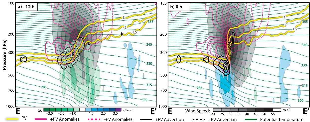
FIG. 10. (a) Cross section along E–E', as indicated in Figs. 8g–i and 12 h prior to an eastern dominant jet superposition. All conventions are identical to those in Fig. 7, with the exception that ascent and descent are shaded in green and blue, respectively, according to the legend in \text{dPa s}^{-1} . (b) As in (a), but for 0 h prior to an eastern subtropical dominant jet superposition.
