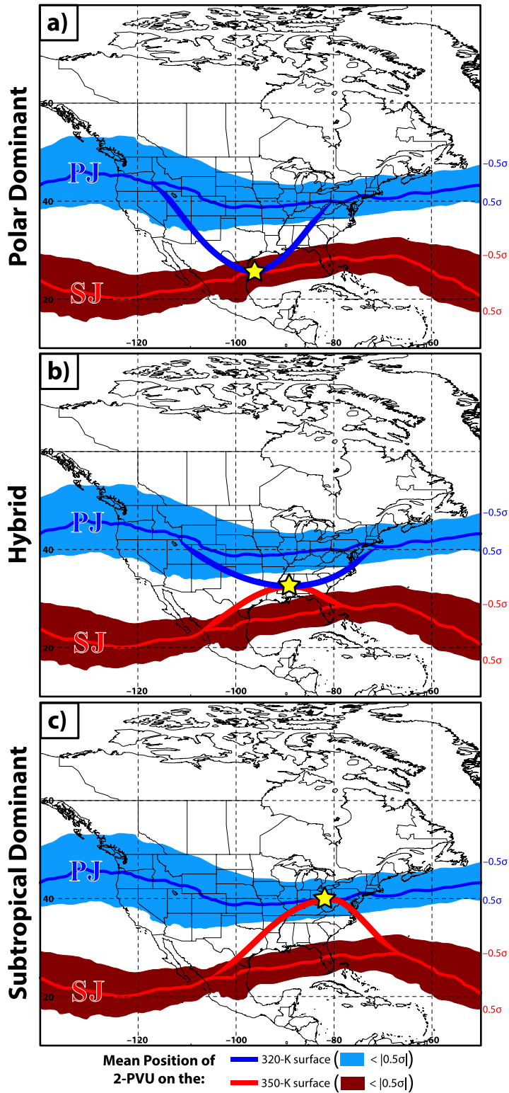
FIG. 2. The mean position of the 2-PVU contour on the 320-K and 350-K surfaces at 0000 UTC 1 Jan is indicated by the thin blue and red line, respectively, as a proxy for the position of the polar (PJ) and subtropical (SJ) waveguide. Shaded areas bounding each mean 2-PVU contour indicate
