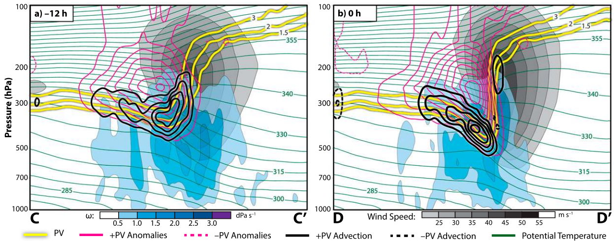
FIG. 7. (a) Cross section along C–C', as indicated in Figs. 5g–i and 12 h prior to a polar dominant jet superposition. Potential temperature (green lines every 5 K), wind speed (gray shading according to the legend in m s -1 ), PV anomalies (magenta lines every 0.5 PVU, solid when positive and dashed when negative), the 1.5-, 2-, and 3-PVU contours (yellow lines), PV advection by the three-dimensional divergent circulation (black lines every 0.5 \times 10^{-5} PVU s -1 , solid when positive and dashed when negative), and descent (blue shading according to the legend in dPa s -1 ). (b) As in (a), but for the cross section along D–D', as indicated in Figs. 5g–i, 0 h prior to a polar dominant jet superposition event.
