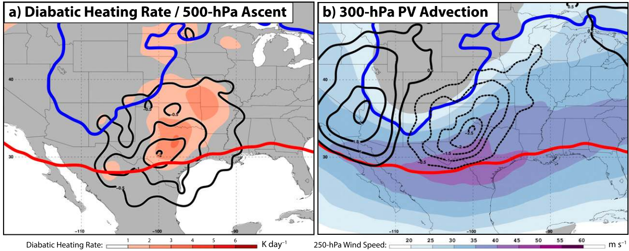
FIG. 6. (a) The 500-hPa diabatic heating rate (shaded according to the legend in K day -1 ), 500-hPa ascent (black lines every -0.5 dPa -1 ), and the position of the 2-PVU contour within the 320–325-K and the 345–350-K layer is indicated by the thick blue and red line, respectively, 24-h prior to a polar dominant jet superposition. (b) As in (a), but with 250-hPa wind speed (shaded according to the legend in m s -1 ), and 300-hPa PV advection by the three-dimensional divergent circulation (black contours every 0.5 \times 10^{-5} PVU s -1 , solid when positive and dashed when negative).
