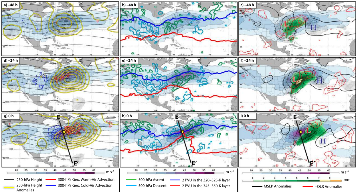
FIG. 8. Composite large-scale flow evolution prior to the initiation of an eastern subtropical dominant jet superposition event. All conventions are identical to those in Fig. 5.
