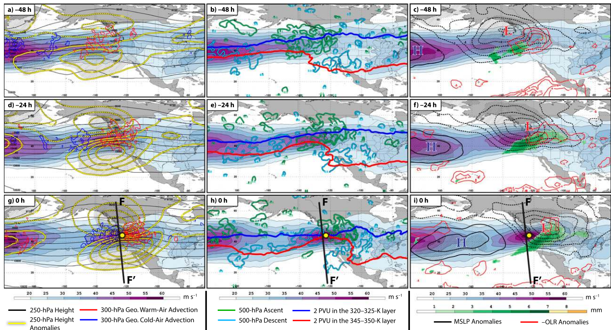
FIG. 11. Composite large-scale flow evolution prior to the initiation of a western subtropical dominant jet superposition event. All conventions are identical to those in Fig. 5.
