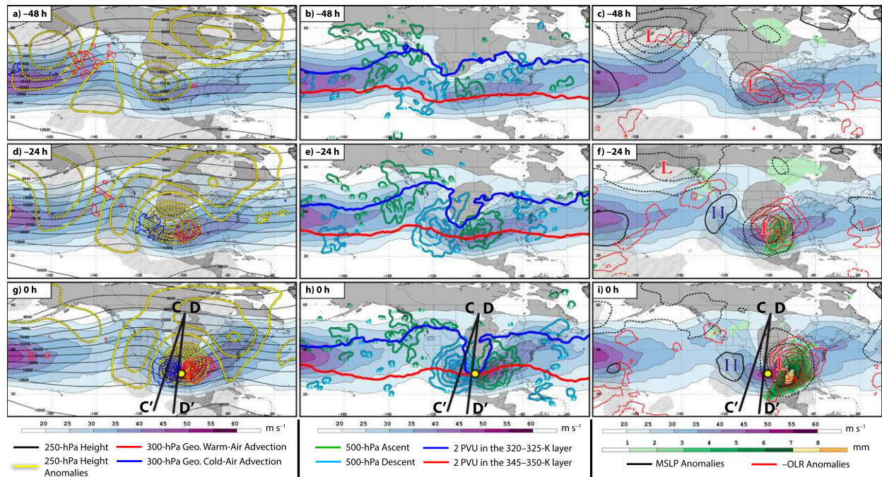
FIG. 5. Composite large-scale flow evolution prior to the initiation of a polar dominant jet superposition event. (left) 250-hPa geopotential height (black solid lines every 120 m), 250-hPa geopotential height anomalies (yellow lines every 30 m, solid when positive and dashed when negative), 250-hPa wind speed (shaded according to the legend in \text{m s}^{-1} ), and 300-hPa geostrophic temperature advection (blue and red lines every 1 \times 10^{-4} \text{K s}^{-1} for cold- and warm-air advection, respectively) for (a) 48 h, (d) 24 h, and (g) 0 h prior to jet superposition. Hatched areas represent locations where the 250-hPa geopotential height anomalies are statistically distinct from climatology at the 99% confidence level. (middle) 250-hPa wind speed (shaded according to the legend in \text{m s}^{-1} ), the position of the 2-PVU contour within the 320–325-K and the 345–350-K layer is indicated by the thick blue and red line, respectively, as a proxy for the location of the polar and subtropical waveguide, and 500-hPa vertical motion (contoured every 0.5 \text{dPa s}^{-1} in green for ascent and in blue for descent) for (b) 48 h, (e) 24 h, and (h) 0 h prior to jet superposition. (right) 250-hPa wind speed (shaded according to the legend in \text{m s}^{-1} ), mean sea level pressure anomalies (black lines every 2 hPa, solid when positive and dashed when negative), negative OLR anomalies (red lines every 4 \text{W m}^{-2} ), and precipitable water anomalies (shaded according to the legend in mm at locations in which the anomalies are statistically distinct from climatology at the 99% confidence level) for (c) 48 h, (f) 24 h, and (i) 0 h prior to jet superposition. Hatched areas represent locations where the mean sea level pressure anomalies are statistically distinct from climatology at the 99% confidence level. The red “L” and blue “H” identify the locations of surface cyclones and anticyclones. The yellow dot in (g), (h), and (i) corresponds to the average location of jet superposition, and the vertical cross sections, C–C’ and D–D’, in (g), (h), and (i) are examined further in Figs. 7a and 7b, respectively.
