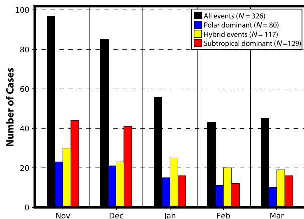
FIG. 3. Monthly frequency of jet superposition events as a function of event type.
