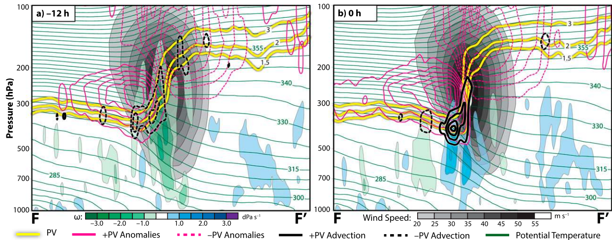
FIG. 13. (a) Cross section along F-F' , as indicated in Figs. 11g–i and 12 h prior to a western subtropical dominant jet superposition event. All conventions are identical to those in Fig. 10. (b) As in (a), but for 0 h prior to a western subtropical dominant jet superposition event.
