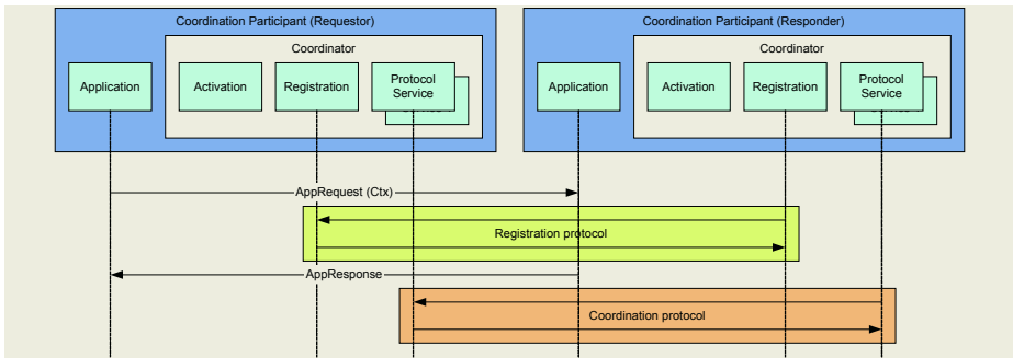
Fig. 3. WS-Coordination Architecture.
