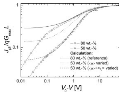
Figure 6. Experimental photocurrent normalized to its saturation value ( qG_{max}L ) as a function of effective applied voltage ( V_0 - V ) for two different OC 1 C 10 -PPV:PCBM compositions (see legend). The lines represent the calculated dissociation probability of bound e-h pairs ( P ) at the donor-acceptor interface as follows: The solid line represents the calculated P that best fits the experimental data, with 80 wt.-% PCBM used as the reference. The dotted line denotes the calculated P for 50 wt.-% PCBM when only the charge-carrier mobilities ( \mu ) have been modified; the dashed line represents the same calculation for the case when both \mu and the bulk dielectric constant ( \epsilon_s ) are modified.
