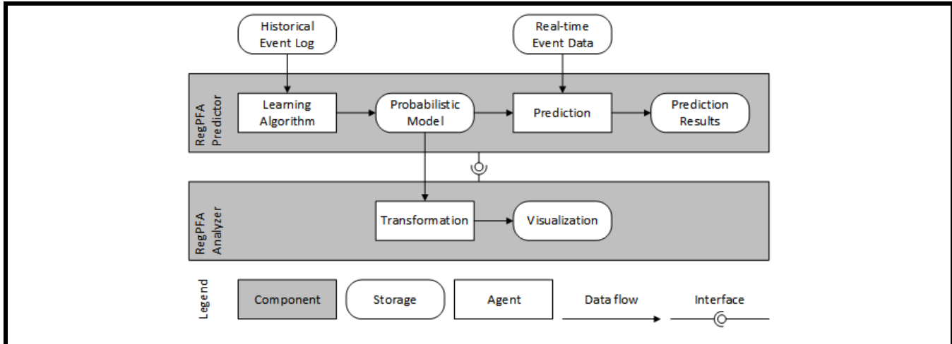
Figure 3. Overview of the RegPFA Artifact
