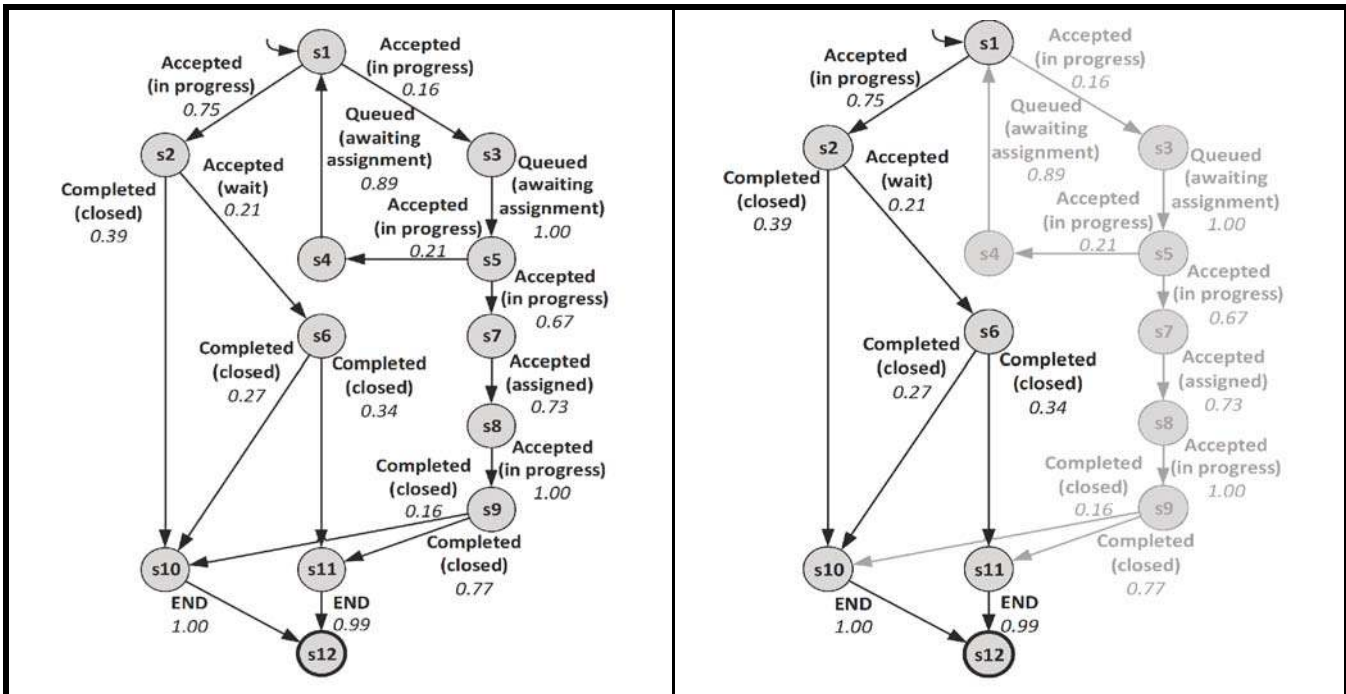
Figure 10. RegPFA Model Visualized with Abstraction Levels of \epsilon = 0.1 (left) and \epsilon = 0.2 (right)
