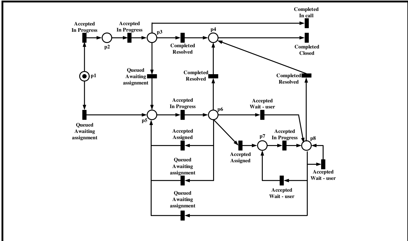
Figure 11. Petri Net Visualization of a Predictive Model for “BPI2013_Incidents”
