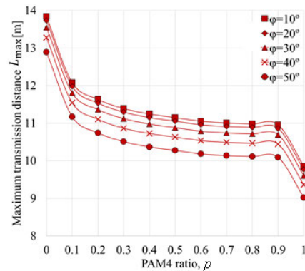
FIGURE 11. Effect of misalignment \varphi on maximum transmission distance L_{\max} for red LD.
