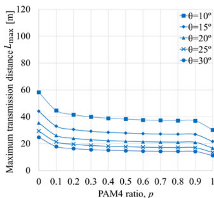
FIGURE 10. Effect on half-beamwidth \theta on maximum transmission distance L_{\max} for blue LD.
