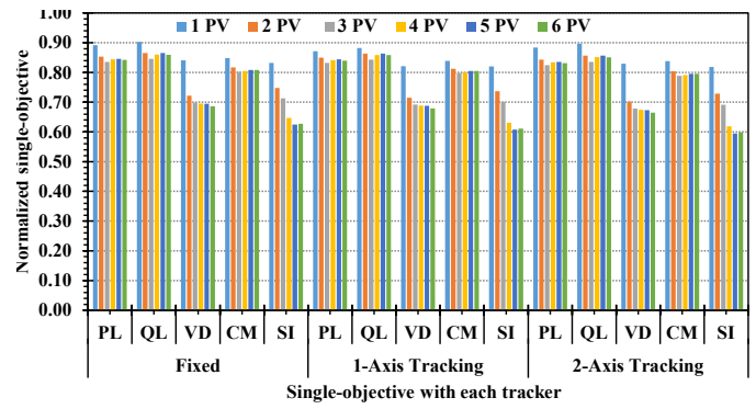
Fig. 3. Single-objective functions for different PV numbers with the three trackers.
