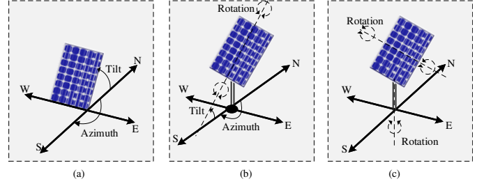
Fig. 1. TOs of PV modules. (a) fixed, (b) one-axis, and (c) two-axis trackers.
