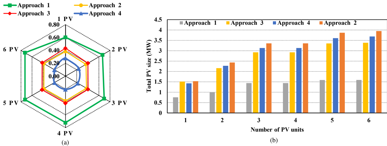
Fig. 8. Results of the PV allocation problem by Approaches 1, 2, 3, and 4. (a) the objective function and (b) total PV size in the distribution system.
