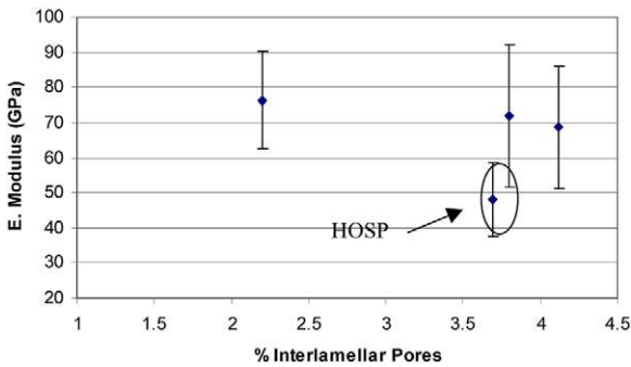
Fig. 11. Porosity–Elastic modulus relationships showing the close connection with interlamellar porosity. Vertical bars indicate the statistical standard deviation in the measured elastic modulus.
