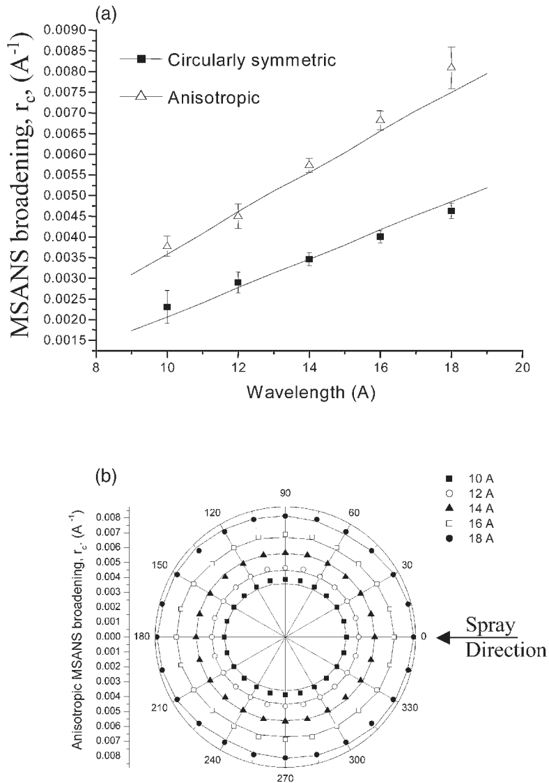
Fig. 7. MSANS broadening experimental data (symbols) with model-fits (lines) for the coating made from F&C feedstock case: (a) MSANS r_c vs \lambda for both the sample orientations; (b) anisotropic angular MSANS, r_c , at different wavelengths
