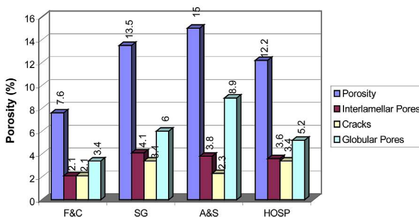
Fig. 8. Quantitative delineation of the coating microstructural features.
