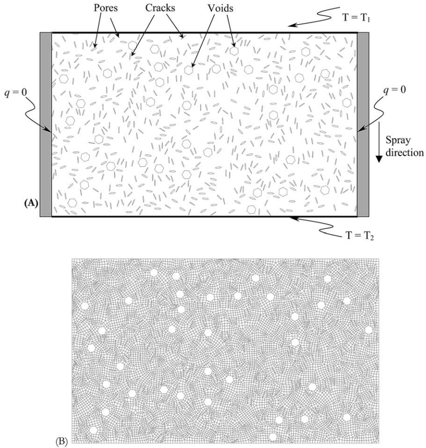
Fig. 13. Computational model of the F&C coating system, with a domain size of 500 \times 300 pixels. (a) Randomly distributed pores, grouped into three types: Cracks, Pores and Voids, with fixed temperatures T_1 and T_2 along the top and bottom boundaries. The heat flux q = 0 indicates no heat loss across boundaries. (b) Finite element mesh, 11500 elements are used.
