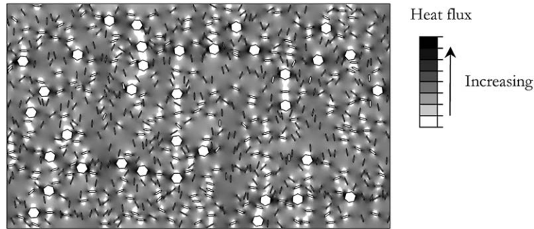
Fig. 14. Contour of heat flux in the spray direction for the coating made from F&C feedstock. Darker areas have higher heat flux.
