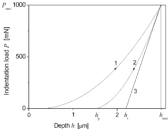
Fig. 3. Force-penetration curve during depth-sensitive microhardness testing. The quantities shown are the depth of indentation at maximum load, h_{max} , the final depth of impression after unloading, h_p , and the intercept of the linear fit, h_r .
