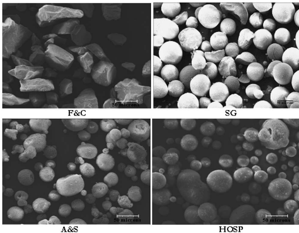
Fig. 1. PSZ powder morphologies observed under SEM (50 \mu\text{m} scalebar).
