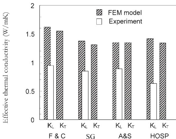
Fig. 15. Comparison of calculated and experimental results of effective thermal conductivity for the four coating systems.
