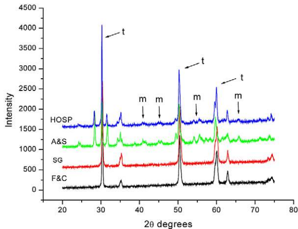
Fig. 2. Phase characterization of powders.
