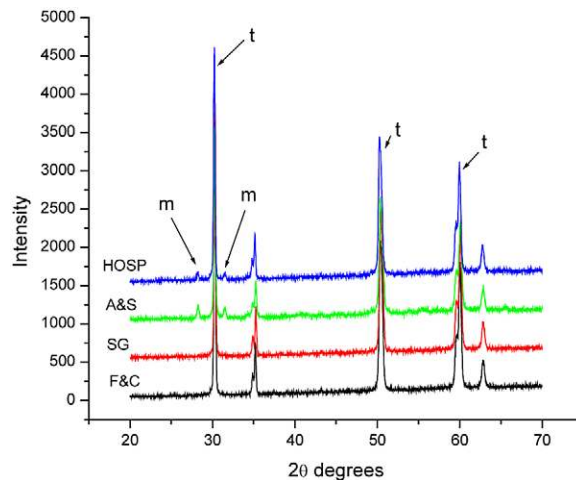
Fig. 5. Phase characterization of coatings.
