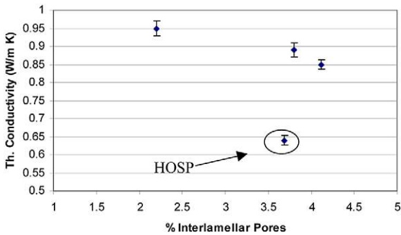
Fig. 10. Porosity–Thermal Conductivity relationships showing the close connection with interlamellar porosity. Vertical bars indicate the statistical standard deviation in the measured thermal conductivity.
