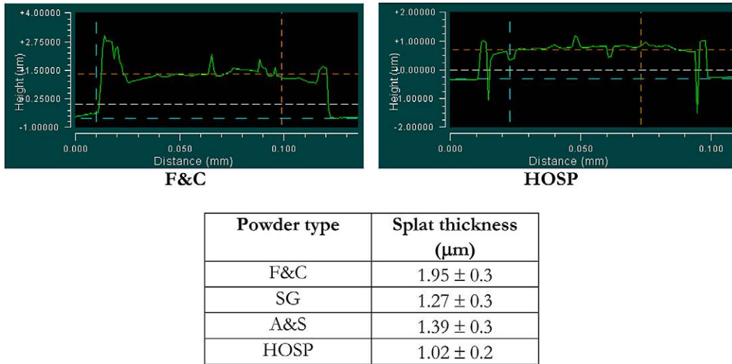
Fig. 12. Figure shows the surface profile of single splat, the dimensions of which are quantified in the table.
