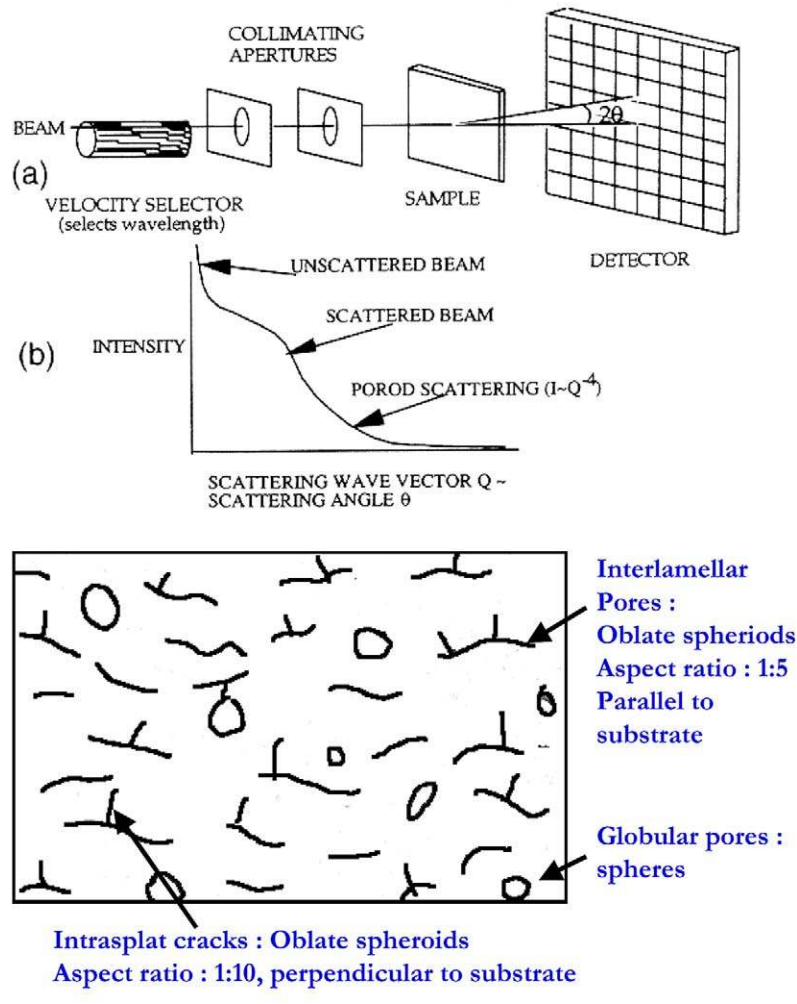
Fig. 4. Experimental setup and scattering intensity curve [16] along with model coating microstructure.
