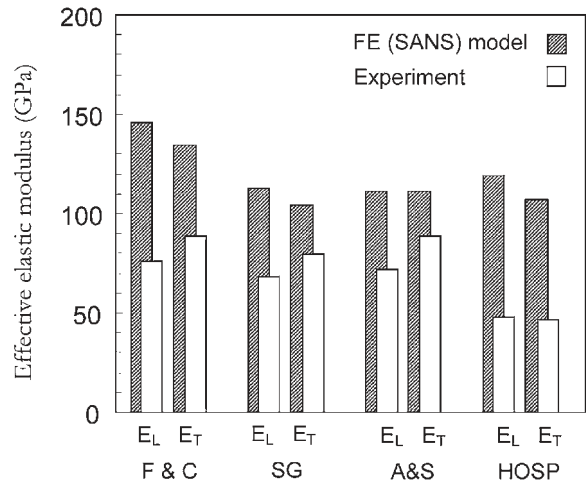
Fig. 16. Comparison of calculated and experimental results of effective elastic modulus for the PSZ coatings.
