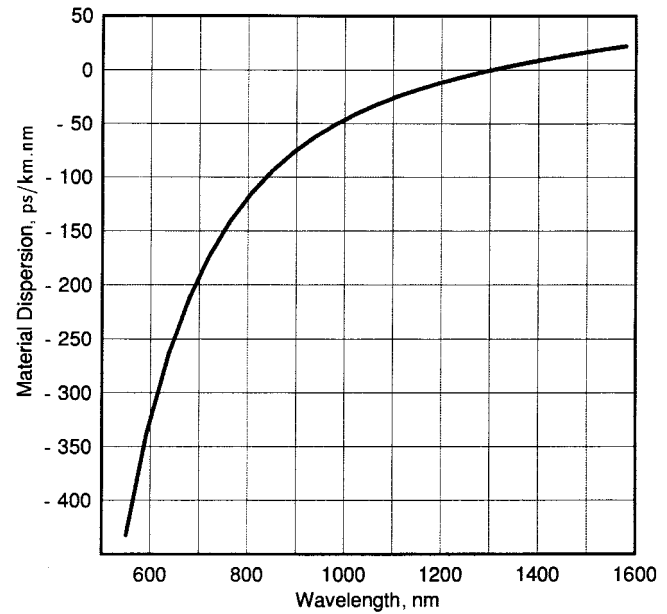
Fig. 2. Material dispersion of the core as a function of wavelength [33].
