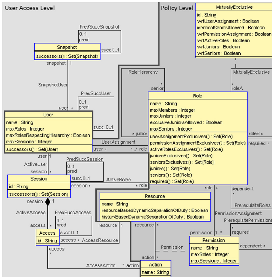
Fig. 6. The RBAC metamodel.
