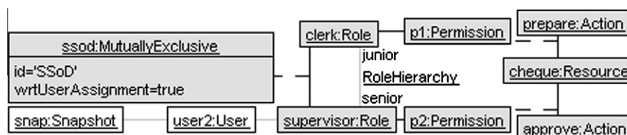
Fig. 8. Partial policy and partial search results (white objects, gray links).
