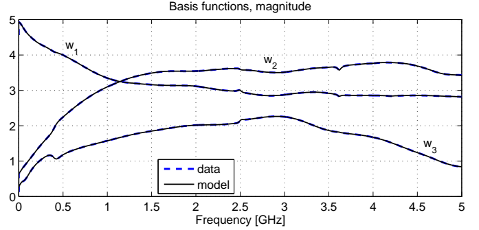
Fig. 2. First three basis functions for case 6. Original frequency samples \tilde{w}_q (dashed lines) and rational model w_q(s) (solid lines).
