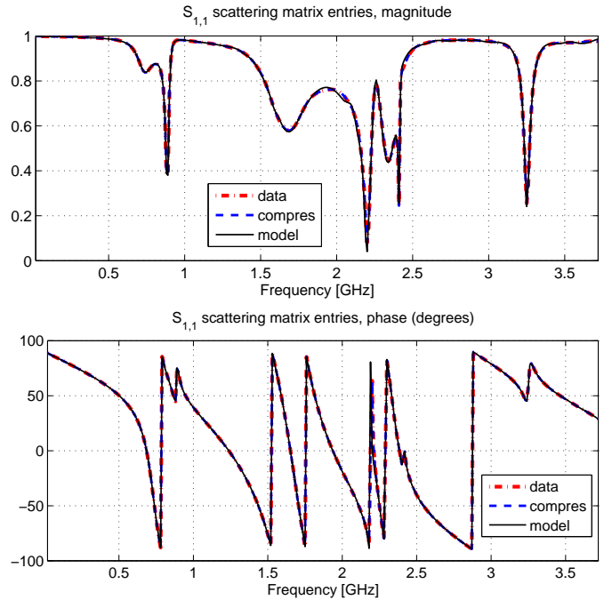
Fig. 4. A scattering response of a PCB interconnect (case 17) before (red dashed line) and after (blue dashed line) compression. The black line represents the response of the passive compressed macromodel.
