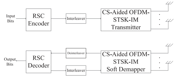
Fig. 3. The transceiver structure of the soft-decision system.
