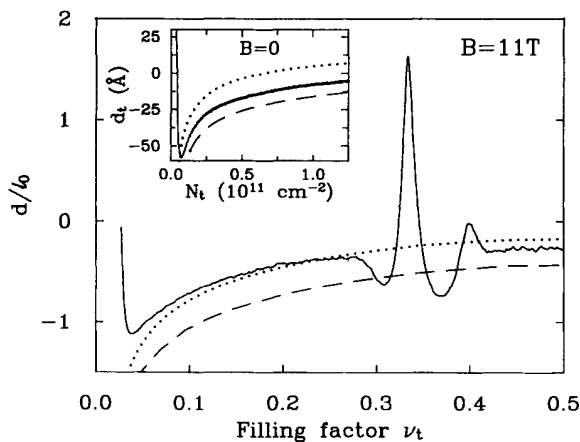
FIG. 7. Compressibility parameter d_t/l_0 vs filling factor \nu_t at B=11 T and T=0.4 K. Dotted curve is the Fano-Ortolani 38 approximation employed by Efros 16 which assumes an ideally thin 2DES. Dashed curve includes the Hartree finite thickness correction but not any softening of the Coulomb interaction. Inset: Analogous comparison at B=0 . Dotted curve represents ideally thin exchange while the dashed curve includes the Hartree correction.
