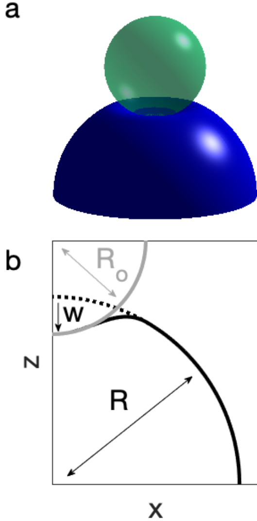
Figure 1: Geometry of the problem: a pressurized spherical shell in contact with a spherical probe. a. Three-dimensional schematic drawing showing the indenter (green, partially transparent sphere) indenting the shell (blue, deformed sphere). b. Cross-section and notations showing the pressurized sphere before indentation (dotted black curve), the pressurized sphere after indentation (continuous black curve) and the rigid spherical probe (grey curve). Here, w is the normal displacement of the probe, while R is the radius of the pressurized sphere and R_o the radius of the rigid sphere (the indenter).
