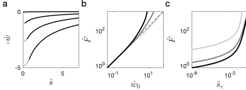
Figure 2: Numerical solutions for the contact of a pressurized spherical shell with a rigid spherical or flat probe. a. Dimensionless displacement \hat{w} as a function of the dimensionless coordinate \hat{s} for \hat{p} = 1 and R/R_o = 1 . The grey (resp. black) part of the line correspond to the contact zone (resp. free zone). b. Dimensionless force as a function of the dimensionless displacement at the origin \hat{w}_0 . The dashed line is a linear fit for small compressions \hat{w} \lesssim 1 . c. Dimensionless force as a function of the dimensionless coordinate, \hat{s}_c , at which contact between the shell and the probe is lost. In (b) and (c), the dimensionless pressure \hat{p} = 8 ; black, dark gray, and gray lines show results for R/R_o = 0 (a plane), R/R_o = 1 , and R/R_o = 10 , respectively.
