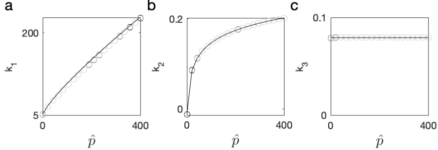
Figure 3: Comparison of analytical and numerical solutions at small displacement. Panels (a), (b), and (c) show the constants k_1 , k_2 , and k_3 that are involved in the equations relating size of contact region, probe displacement, and force, respectively, plotted as functions of the dimensionless pressure, \hat{p} . Circles represent the constants estimated from fits to numerical solutions and while curves show the predictions of the analytical solution of the linearized equations. Black, dark gray, and gray circles stand for R/R_o = 0 (a plane), R/R_o = 1 , and R/R_o = 10 , respectively.
