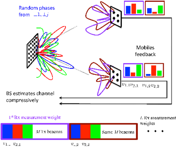
Fig. 2: Channel sounding scheme: The transmitter repeats the M transmit beacons L times so that receivers can measure the channel v_{i,j} between every virtual transmit-receive pair
