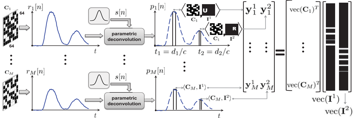
Figure 2. Depth map reconstruction algorithm. The intensity samples r_i[n] acquired for each binary pattern C_i are first processed using parametric deconvolution to recover scene response p_i[n] . The positions of peak amplitudes in p_i[n] provide depth estimates, d_1 and d_2 , and the amplitudes are used to recover the spatial structure of the depth map (i.e. the depth masks \mathbf{I}^1 and \mathbf{I}^2 ) at these depth locations. The spatial resolution is recovered by a convex program that enforces gradient-domain sparsity and includes a robustness constraint.
