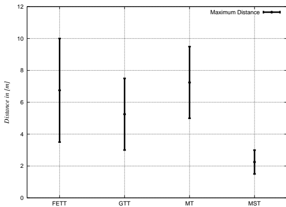
Figure 18: Maximum distance ranges, from the least vulnerable keyboard to the most vulnerable keyboard, to successfully recover 95% of the keystroke according to the techniques (in the office with the biconical antenna).
