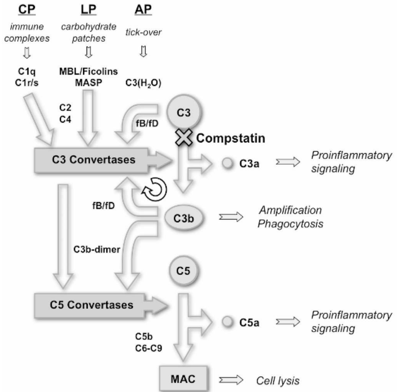
Fig. 1. Compstatin inhibits the cleavage of native C3 to its active fragments C3a and C3b. As a consequence, the deposition of C3b, the amplification of the alternative pathway and all downstream complement actions are prevented
