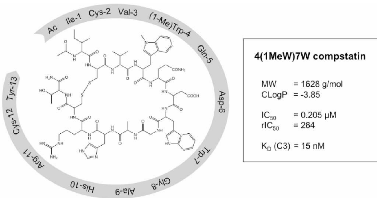
Fig. 4. Optimized lead structure of compstatin (Ac-ICV(1MeW)QDWGAHRCT-NH 2 ) with key biophysical properties. The tridecapeptide chain is synthesized using solid phase peptide synthesis and cyclized via a disulfide bond between the cysteine residues at positions 2 and 12. The IC 50 values represent inhibition of the classical pathway of complement activation both as absolute value and relative to the original compstatin
