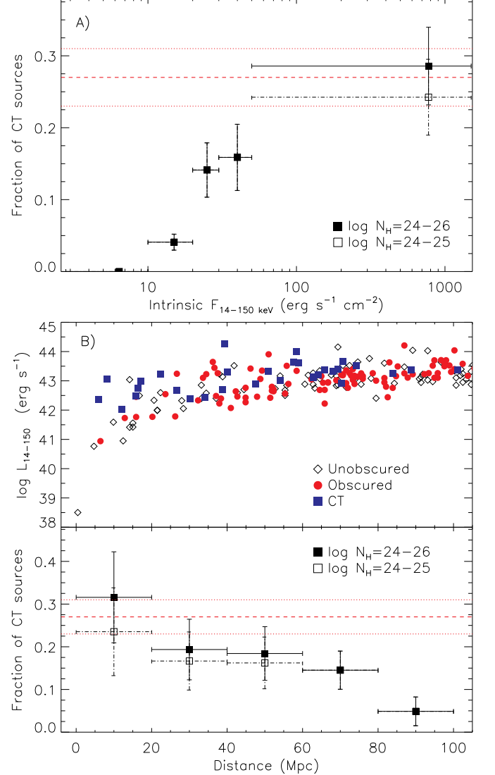
Figure 3. Panel A: Fraction of CT AGN versus the intrinsic (i.e. absorption-corrected) 14–150 keV flux. Panel B: Intrinsic 14–150 keV luminosity ( top panel ) and observed fraction of CT sources ( bottom panel ) versus distance for the AGN located within 100 Mpc. The decrease of the observed CT fraction with the decreasing intrinsic flux and the increasing distance is due to the observational bias of the Swift /BAT survey against sources with \log N_H > 24 . In both panel A and B the empty and filled points represent the fraction of AGN with \log N_H = 24 - 25 and \log N_H = 25 - 26 , respectively. The red dashed line shows the intrinsic fraction of sources with \log N_H = 24 - 25 ( 27 \pm 4\% , see Sect. 4), while the red dotted line is the associated uncertainty.
