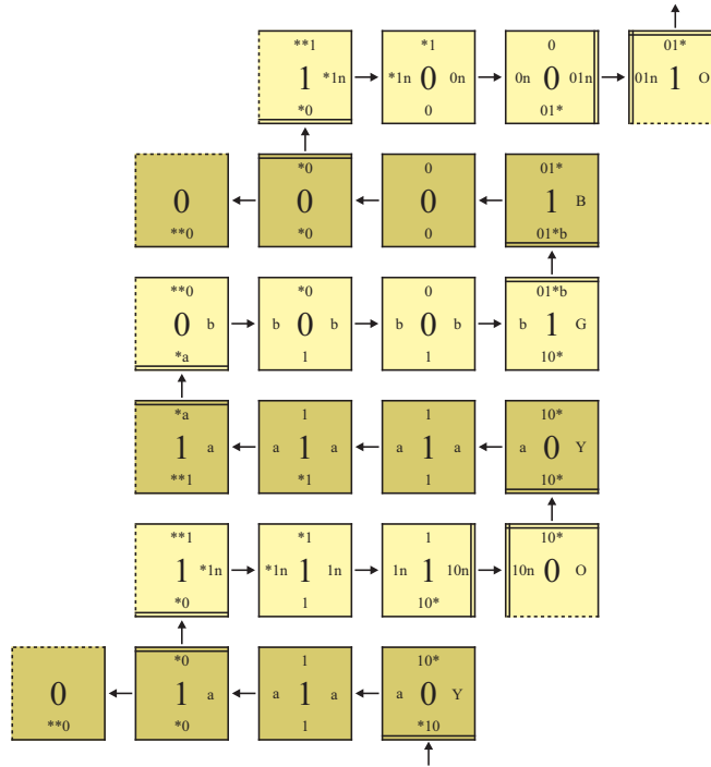
Fig. 3. If the current value of the binary counter is a power of 2 (the fourth row of tiles), then the increment row that represents this value does not shift to the right by one unit. This situation is detected in the third (copy) row by the ‘a’ signal, which travels unimpeded right-to-left. The complementary ‘b’ signal is then sent left-to-right in the subsequent increment row to initiate a green signal.
