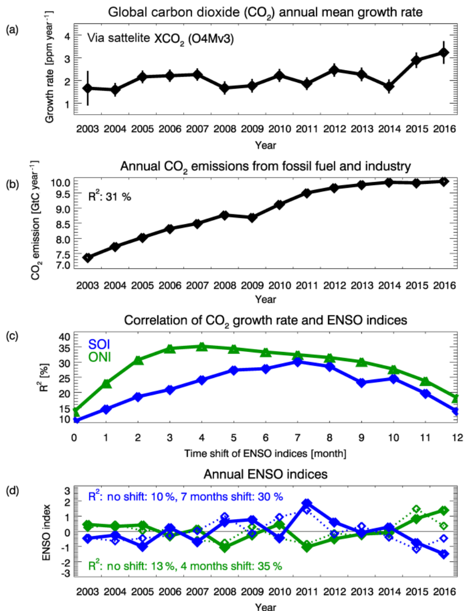
Figure 3. Carbon dioxide global annual mean growth rates compared with human emissions and ENSO indices. (a) Satellite-derived global annual mean growth rates (with 1\sigma uncertainty range shown as vertical lines). (b) CO 2 emissions from fossil fuel and industry (the correlation with the growth rate is R^2 = 31\% ). (c) Correlation in terms of R^2 of growth rate and annual SOI (blue curve) and ONI (green curve) as a function of time shift in months. (d) Annual SOI for no shift (blue dotted line, R^2 = 10\% ) and for a shift of 7 months (blue solid line, R^2 = 30\% ) and annual ONI for no shift (green dotted line, R^2 = 13\% ) and for a shift of 4 months (green solid line, R^2 = 35\% ).
