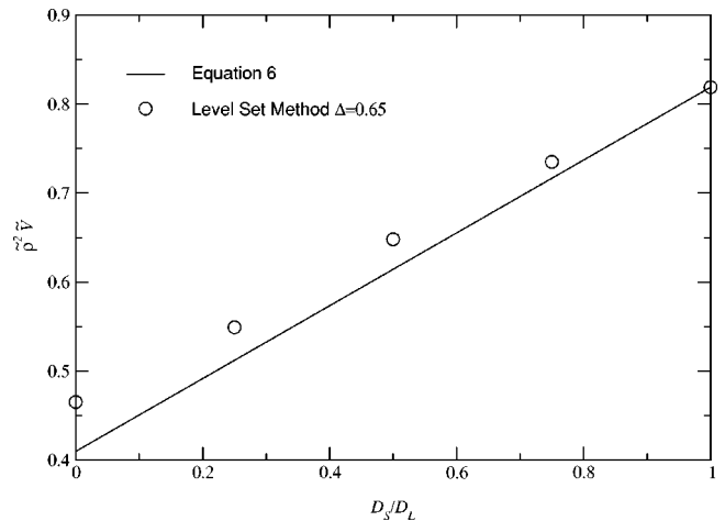
FIG. 3. \bar{\rho}^2 \bar{V} for different values of D_S/D_L . The circles are data from level set simulations at \Delta = 0.65 . The solid line is the theoretical prediction of Barbieri and Langer fitted to the data point at D_S/D_L = 1 .
