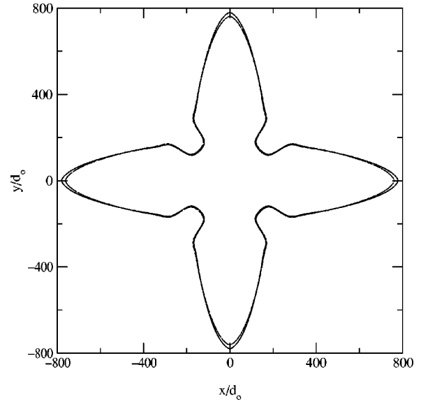
FIG. 2. Comparison of dendritic shapes computed from the level set method and phase-field model for \Delta = 0.55 , shown at \tilde{t} = 37\,600 .
