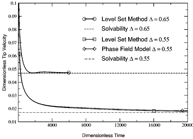
FIG. 1. Time evolution of the dimensionless tip velocity for simulations at \Delta = 0.65 and 0.55 .
