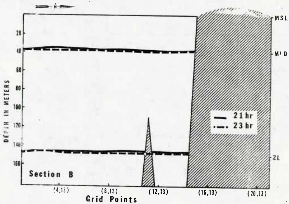
Figure 39. Depth of layer interfaces along sections A and B during and 2 hours after secondary high water at Long Beach.
