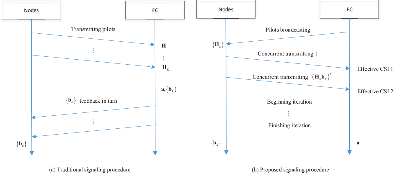
Figure 2. The signaling procedure of transceiver optimization of CoMAC.
