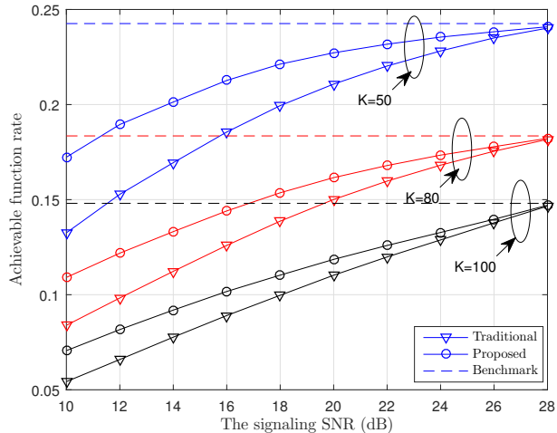
Figure 11. The achievable function rate versus different number of nodes in multi-cluster network.
