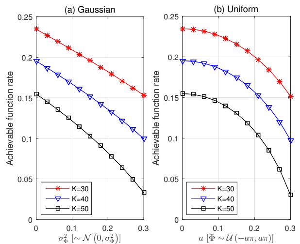
Figure 12. The sum computation rate versus different number of nodes in multi-cluster network.
