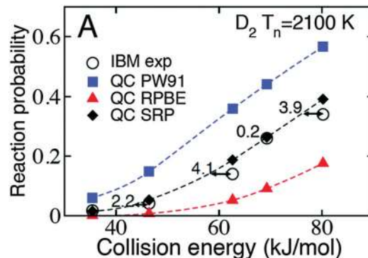
Fig. 6 S_0 computed 43 with the QCT method (QC in legend) using the PW91, 312 RPBE, 196 and SRP43 43 (SRP) DFs are compared with experimental 12 values for D_2 + Cu(111) (IBM exp). The computed S_0 exhibit statistical errors \leq 0.005 . Figure taken from ref. 43.
