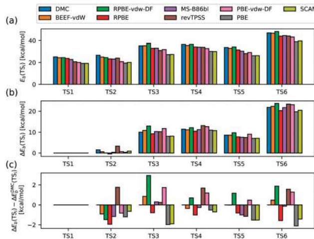
Fig. 8 (a) Comparison of barrier heights E_b computed 429 for H 2 + Al(110), for six geometries (TS1–TS6) sampling different impact sites and orientations with DMC and DFT using 8 different density functionals. (b) Similar as in (a), but now plotting \Delta E_b(\text{TS}_i) = E_b(\text{TS}_i) - E_b(\text{TS}_1) for i = 1-6 , for each method. (c) Similar to (b), but now plotting \Delta E_b(\text{TS}_i) - \Delta E_b^{\text{DMC}}(\text{TS}_i) for each method. Reprinted from [A. Powell, G. J. Kroes and K. Doblhoff-Dier, Quantum Monte Carlo calculations on dissociative chemisorption of H 2 on Al(110): minimum barrier heights and their comparison to DFT values, J. Chem. Phys. , 2020, 153 , 224701], with the permission of AIP Publishing.
