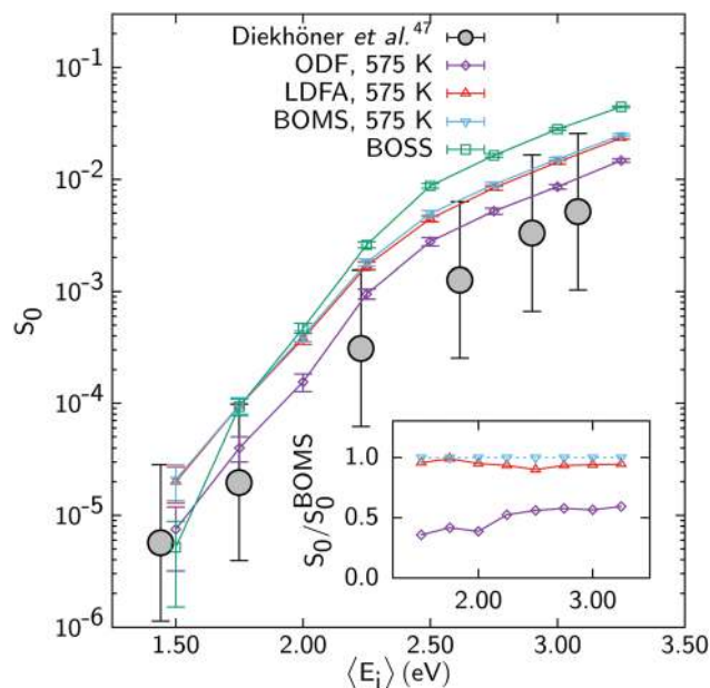
Fig. 14 S_0 computed for N 2 + Ru(0001) with MDEF and the RPBE DF using the BOSS model, 139 the BOMS model, 139 and the NBOMS model with the LDAF and the ODF approximations 59 are shown as a function of E_i . Experimental results are also shown. Taken from ref. 59 ( https://pubs.acs.org/doi/10.1021/acs.jpcclett.9b00523 ). Further permission requests to be directed to the ACS.
