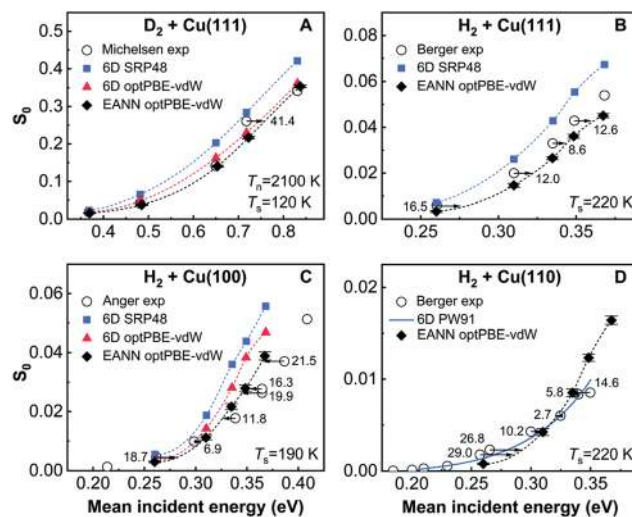
Fig. 39 S_0 computed with PESSs based on the optPBE- vdW1 DF for D_2 + Cu(111) (A), H_2 + Cu(111) (B), H_2 + Cu(100) , and H_2 + Cu(110) with high-dimensional QCT calculations are compared with molecular beam sticking experiments 12,649,667,730 on these systems. Black arrows and accompanying numbers (in meV) indicate the incident energy spacing between the experimental and interpolated computed curves. Reproduced from ref. 467 with permission from the PCCP Owner Societies.
