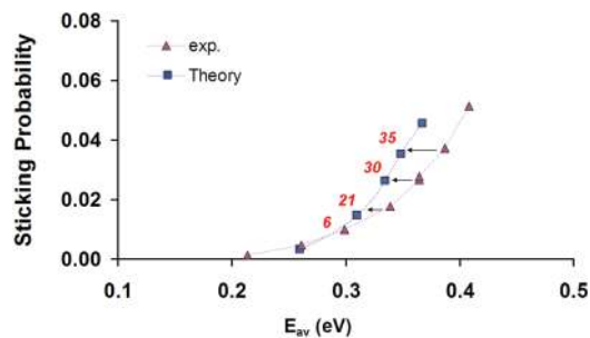
Fig. 37 Measured 667 and computed 46 S_0 are shown as a function of average normal incidence energy for sticking of H_2 on Cu(100) . The dynamics calculations were performed 46 with the TDWP method and used a PES computed with the original SRP DF 43 derived for H_2 + Cu(111) . The numbers shown represent the energy difference in meV between the values of the measured S_0 and the cubic spline interpolated theoretical S_0 curve. Reprinted from [L. Sementa, M. Wijzenbroek, B. J. van Kolck, M. F. Somers, A. Al-Halabi, H. F. Busnengo, R. A. Olsen, G. J. Kroes, M. Rutkowski and C. Thewes, et al. , Reactive scattering of H_2 from Cu(100) : comparison of dynamics calculations based on the specific reaction parameter approach to density functional theory with experiment, J. Chem. Phys. , 2013, 138 , 044708], with the permission of AIP Publishing.
