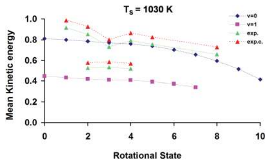
Fig. 38 Calculated 46 (“ v = 0 ” and “ v = 1 ” and measured 46 (“exp.”) ADEs are shown as a function of the rotational state J of H_2 desorbing from Cu(100) at T_s = 1030 K. The “exp.c” results were approximately corrected for the use of a static 0 K surface in the calculations. 46 Reprinted from [L. Sementa, M. Wijzenbroek, B. J. van Kolck, M. F. Somers, A. Al-Halabi, H. F. Busnengo, R. A. Olsen, G. J. Kroes, M. Rutkowski and C. Thewes, et al. , Reactive scattering of H_2 from Cu(100) : comparison of dynamics calculations based on the specific reaction parameter approach to density functional theory with experiment, J. Chem. Phys. , 2013, 138 , 044708], with the permission of AIP Publishing.
