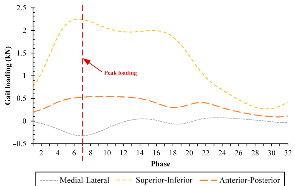
Figure 3. Triaxial forces under gait cycle [24].
