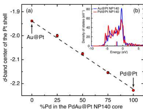
Figure 3. (a) Average d -band center (red circles) of the Pt shell varying linearly with the fraction of Pd in the alloy-core, x , in \text{Pd}_x\text{Au}_{1-x} @Pt NP140. (b) d -band density of states for the Pt shell at the two end point structures: Au@Pt (blue) and Pd@Pt (red) NP140. The small vertical marks above the x axis indicate the center of the d -bands. The Pd core lowers the d -band of the Pt shell in comparison with the Au core.
