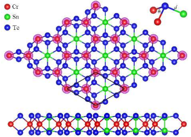
FIG. 1. Top and side views of single-layer \text{CrSnTe}_3 structure. The solid black line encloses a unit cell of single-layer \text{CrSnTe}_3 . The spin charge density is also shown with an iso-surface of 0.025 e/\text{\AA}^3 .
