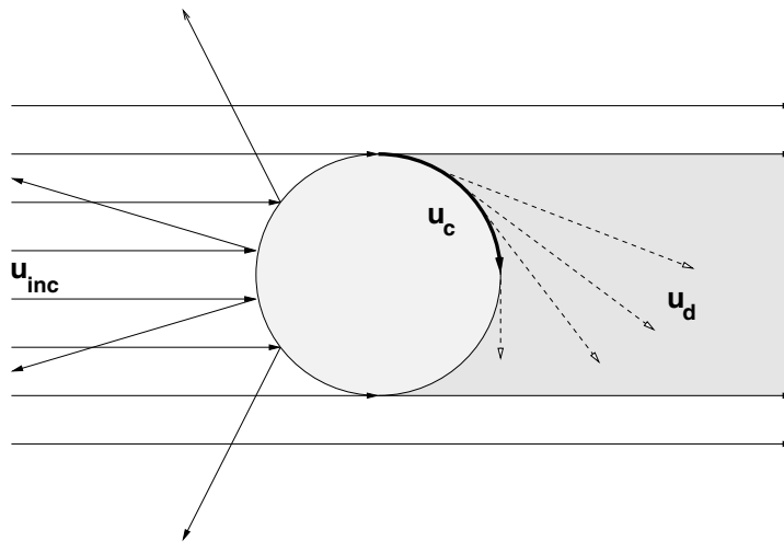
Figure 2.4. Diffraction by a smooth cylinder. The incident field u_{inc} induces a creeping ray u_c at the north (and south) pole of the cylinder. As the creeping ray propagates along the surface, it continuously emits surface-diffracted rays u_d with exponentially decreasing initial amplitude.
