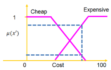
Figure 3.12. The membership functions for cost
