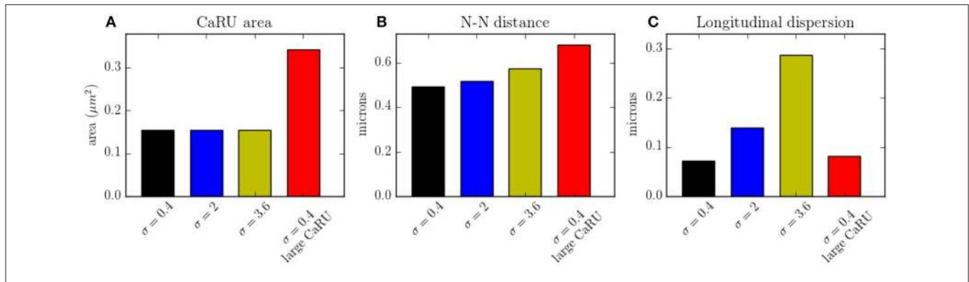
FIGURE 14 | (A) Mean area occupied by a CaRU. (B) Nearest-neighbor distance among CaRUs, measured from the center of each CaRU. (C) Longitudinal dispersion, measured as the mean distance between the RyRs and the center of the z-line. All calculations have been averaged over 35 configurations.
