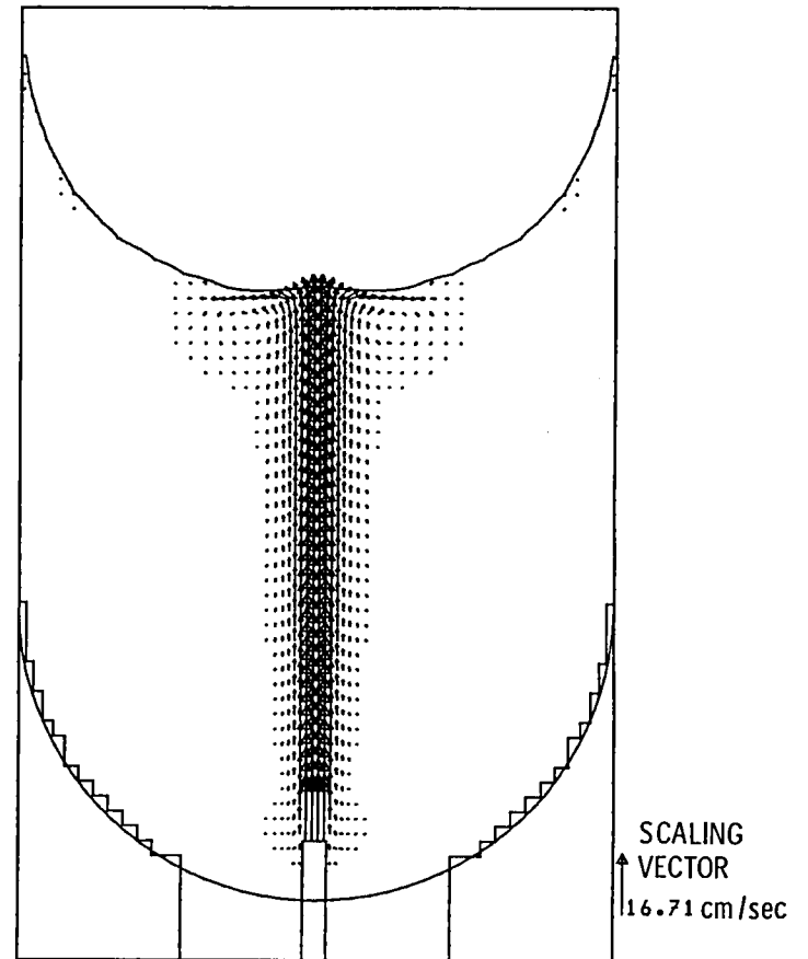
Figure 4. - Calculated velocity field with laminar jet after 2 sec (3894 computational cycles).
