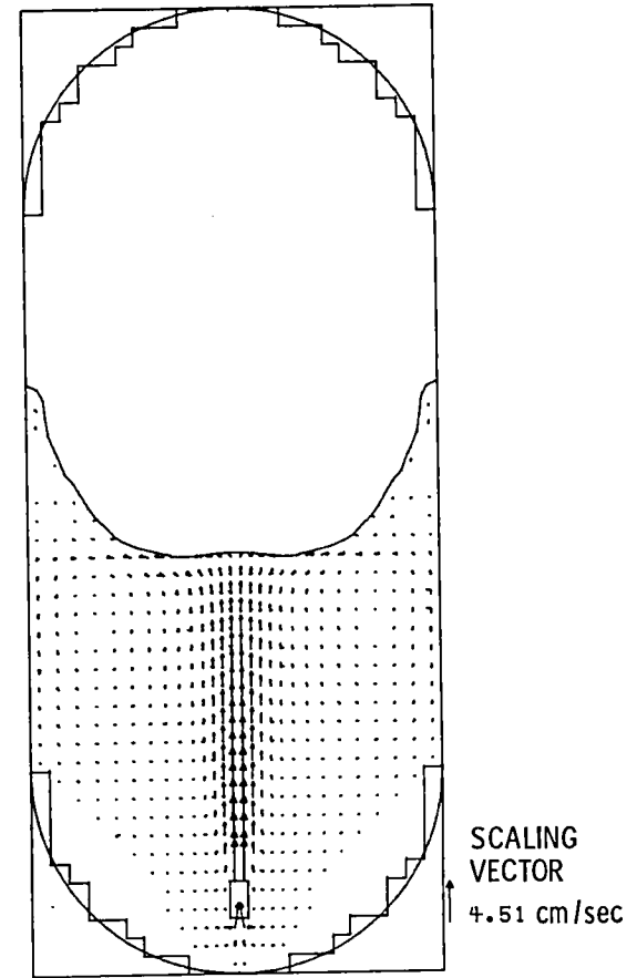
Figure 14. - Calculated velocity field for OTV liquid hydrogen tank with turbulent jet after 2 hr (14244 computational cycles).
