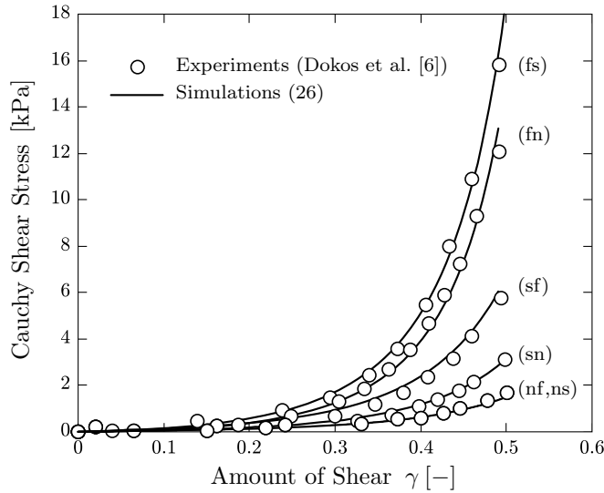
Figure 3. Experimentally measured [6] and computationally predicted stress-strain curves for the six simple shear experiments depicted in Figure 2. The identified material parameters are given in Table I.
