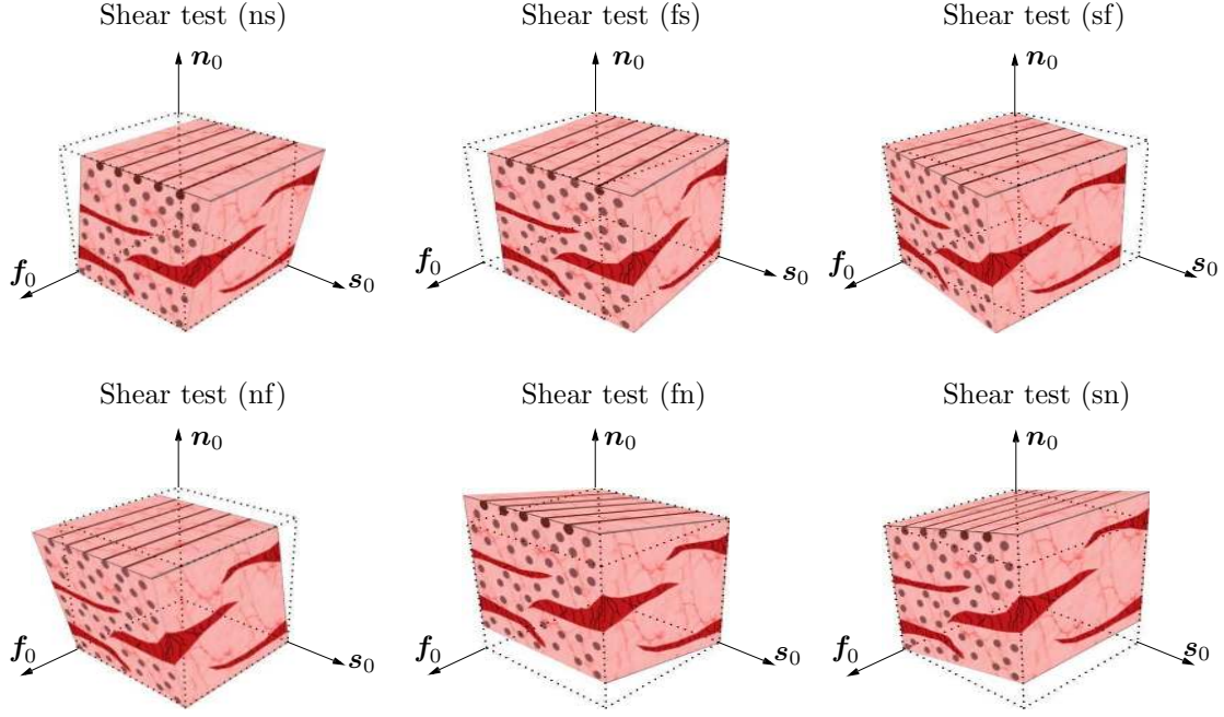
Figure 2. Schematic illustration of the six shear experiments [6] serving as data base for the parameter identification. The stress-strain curves corresponding to these shear modes are depicted in Figure 3.
