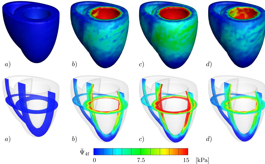
Figure 5. The contour plots of the fiber stress coefficient \bar{\Psi}_{4f} on the solid model (upper row) and on the slices located at x = 0 and z = 25 mm (lower row). The labeling a) – d) of the snapshots is consistent with the chosen four representative stages of the pressure transient, given in Figure 4.
