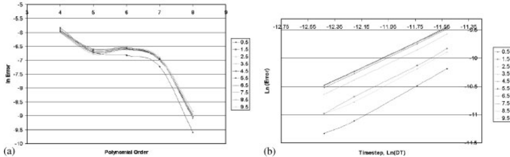
Figure 15. Logarithmic plot of velocity error at a point in the abdominal aorta (artery 39) against: (a) polynomial order and (b) timestep.
