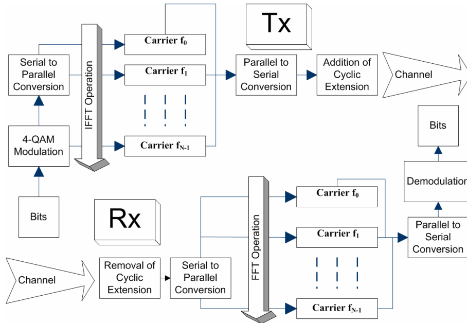
Figure 1. OFDM system model.
