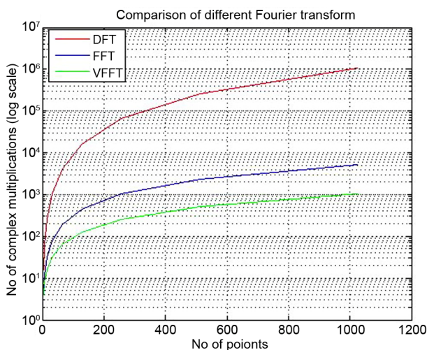
Figure 2. Comparison of different fourier transforms (multiplications only).
