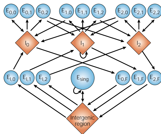
Figure 5 | A generalized pair hidden Markov model. A generalized pair hidden Markov model (GPHMM) for aligning and predicting exons using genomic DNA sequences from two related organisms. The main difference between this model and the usual HMM (such as Genscan) is that an exon pair (one from each organism) is generated according to some joint distribution. ‘E’ represents an exon-pair state. The internal exon pairs are shown at the top. E_{ij} indicates the state that can create an exon-pair connecting an upstream i -phase intron ( I_i ) and a downstream j -phase intron ( I_j ) (where i, j = 0, 1 or 2 ). E_{i1} indicates the first exon state that can create an initial exon-pair that connects a downstream i -phase intron, and E_{i2} indicates the last exon-pair state that can create a final exon-pair that connect to an upstream j -phase intron. E_{sing} indicates a simple exon state (an intronless gene). Modified with permission from REF. 79 © (2002) Mary Ann Liebert, Inc.
