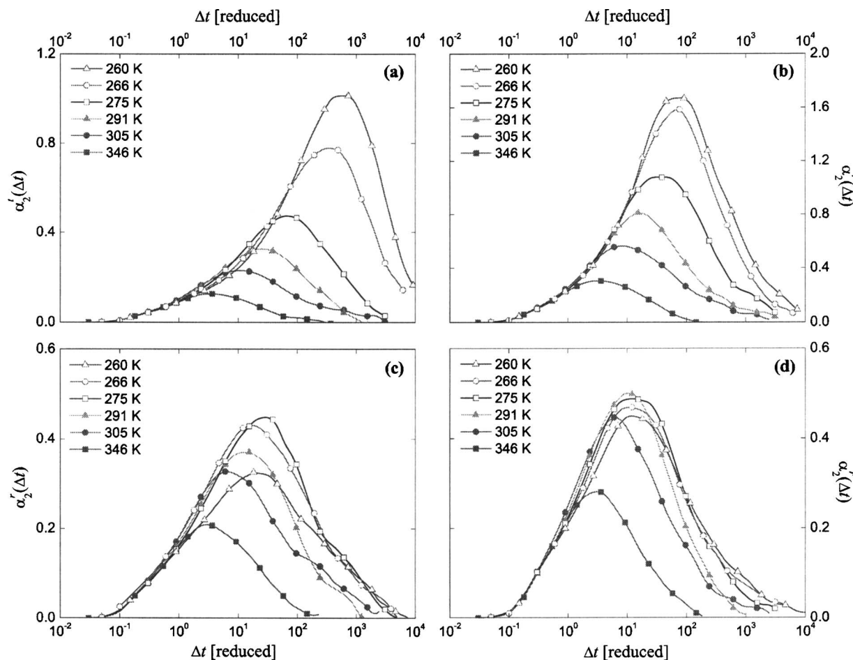
FIG. 3. The non-Gaussian parameters, \alpha_2^x and \alpha_2^y , for (a) translation in one dimension and (b) rotation in the \varphi^x , (c) \varphi^y , and (d) \varphi^z directions. The time at which \alpha_2^x and \alpha_2^y attain their maximum value corresponds to \Delta t^* .
